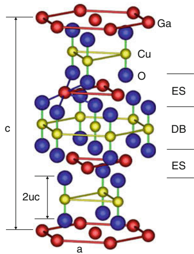
Fig. 3.25 Hexagonal unit cell of delafossite CuGaO 2 . Oxygen atoms are bonded to the Cu in a dumbbell (‘DB’) configuration. In the edge-sharing (‘ES’) layer the Ga atoms are octahedrally configured as GaO 6
