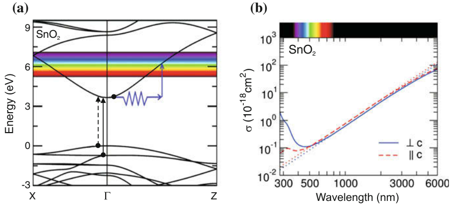
Fig. 9.46 (a) Band structure of \text{SnO}_2 and absorption processes; the transition from the topmost valence band ( dashed arrow ) is forbidden. (b) Calculated free-carrier absorption ( \sigma = \alpha/n ) for \text{SnO}_2 . The solid and dashed lines are results including phonon-assisted transitions for two light polarizations. The dotted lines are fits of the Drude model to the infrared regime. Adapted from [814]
