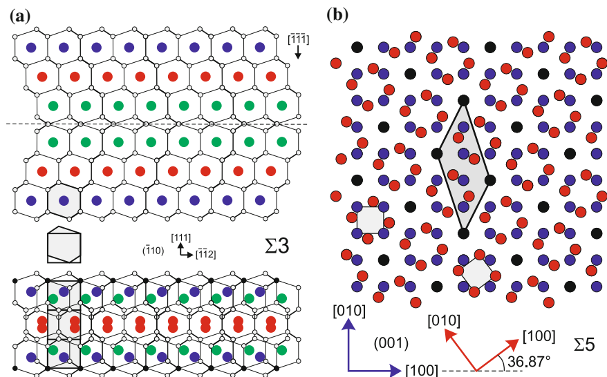
Fig. 4.33 (a) Schematic of \Sigma 3 (111) twin boundary in a diamond or zincblende structure (cmp. Fig. 4.28). The grain boundary is marked by a dashed line shown in side-view. The hexagonal and rectangular grey boxes have the same area. The lattice points of the coincident site lattice (CSL) are shown with black circles in the lower part of the figure. The unit cell of the CSL has three times the volume of the unit cell of the fcc lattice. (b) Schematic of a \Sigma 5 (001) grain boundary in a (simple) cubic crystal shown in plane-view. The blue and the red lattice are rotated by 36.86^\circ , the lattice points of the CSL are shown in black . The unit cell of the CSL lattice ( dark grey ) has five times the volume of the cubic unit cell ( light grey )
