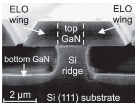
Fig. 12.14 SEM cross-sectional image of GaN grown on a structured Si(111) substrate. The laterally grown wings extend about 2.5\text{ }\mu\text{m} over the grooves. The thickness of the GaN layer is 0.5\text{ }\mu\text{m} on the bottom of the grooves, while it is 1.4\text{ }\mu\text{m} on top of the ridges. Reprinted with permission from [1013], © 2001 AIP
