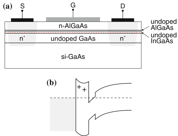
Fig. 24.46 (a) Scheme of a PHEMT structure with n-AlGaAs/InGaAs heterointerface on semi-insulating GaAs. The source and drain contacts are n-doped such that this structure can be used as an n-channel HEMT. The horizontal dashed line represents schematically the position of the 2DEG in the InGaAs layer. (b) Band diagram at zero gate voltage
