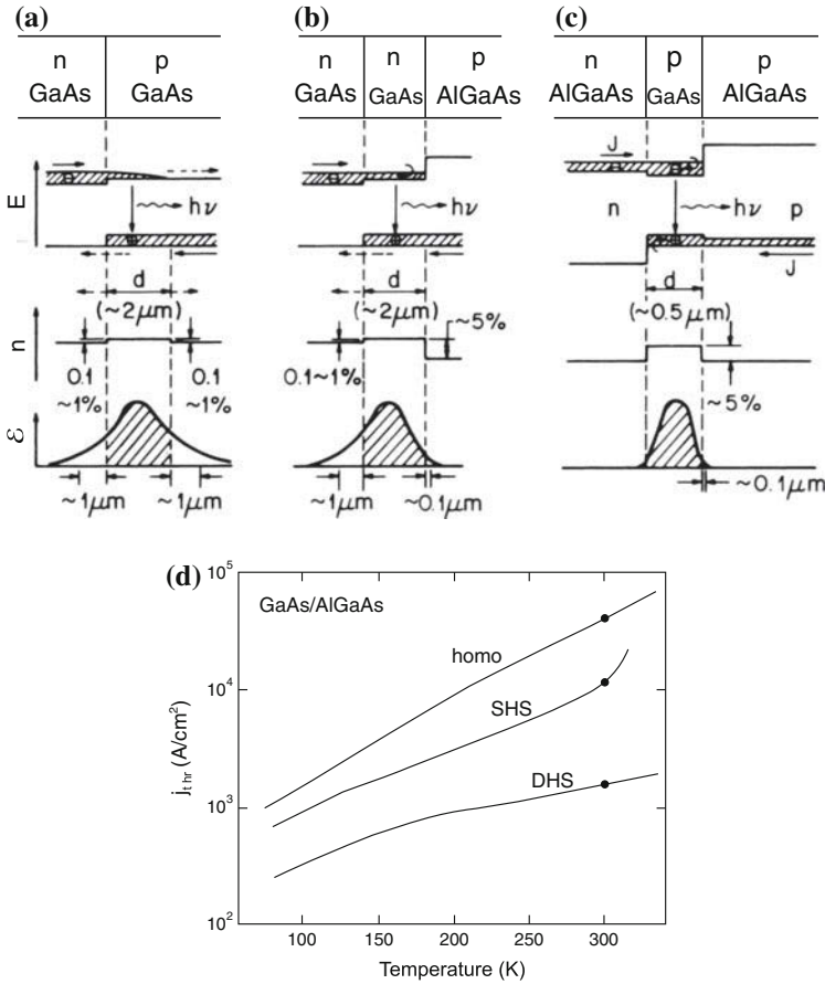
Fig. 23.36 Laser with (a) homojunction, (b) single heterostructure (SHS), (c) double heterostructure ('DHS'), (d) reduction of threshold current with design progress ('SHS': d = 2\mu\text{m} , 'DHS': d = 0.5\mu\text{m} ). Adapted from [1682]
