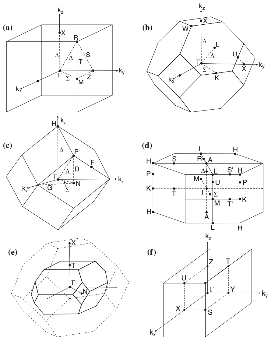
Fig. 3.34 Brillouin zones and special \mathbf{k} points for the (a) primitive cubic (pc), (b) fcc, (c) bcc, and (d) hcp lattice. (e) Brillouin zone for chalcopyrite structure with fcc Brillouin zone shown as dashed outline. (f) Brillouin zone for orthorhombic lattice with one quadrant shown with dashed lines.
