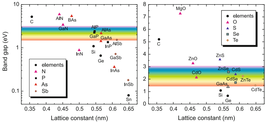
Fig. 6.16 Band gaps as a function of the lattice constant for various elemental, III–V and II–VI semiconductors. The lattice constant of wurtzite semiconductors has been recalculated for a cubic cell
