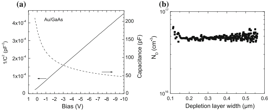
Fig. 21.10 (a) Capacitance C (dashed line) and 1/C^2 (solid line) versus bias voltage dependence for an Au/GaAs Schottky diode (2- \mu\text{m} MOVPE-grown GaAs:Si on a n-GaAs substrate) at room temperature. From the extrapolation to 1/C^2 = 0 and (21.30) we obtain V_{\text{bi}} = 804 \pm 3 \text{ mV} . (b) Donor concentration ( N_D = 4.8 \times 10^{16} \text{ cm}^{-3} ) determined via (21.31) from the 1/C^2 plot versus the depletion layer width (calculated using (21.29))
