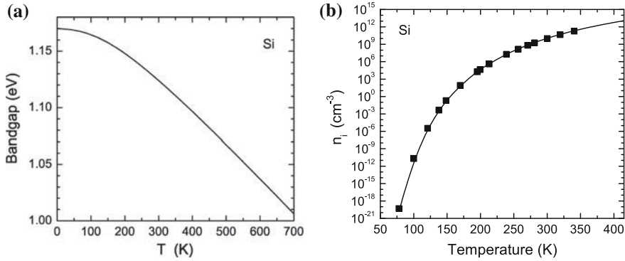
Fig. 7.3 (a) Band gap of silicon versus temperature. (b) Intrinsic carrier concentration of silicon versus temperature. Solid line is (7.17) using E_g = 1.204 \text{ eV} - (2.73 \times 10^{-4} \text{ eV/K}) T [491], symbols are experimental data from [492]
