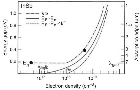
Fig. 9.40 Burstein–Moss effect at InSb ( E_g = 0.18 eV) at room temperature. Theoretical dependence and data points for intrinsic InSb and 5 \times 10^{18} \text{ cm}^{-3} n-type. Data from [806]
