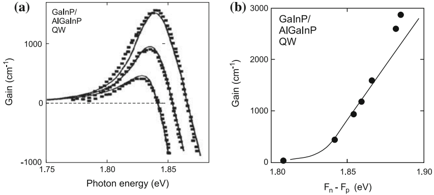
Fig. 23.35 (a) Gain spectra of a 6.8 nm thick \text{Ga}_{0.41}\text{In}_{0.59}\text{P}/(\text{Al}_{0.5}\text{Ga}_{0.5})_{0.51}\text{In}_{0.49}\text{P} quantum well, experimental data ( symbols ) and theory ( lines ) for three different sheet carrier densities n_{2\text{D}} = 2.2, 2.7, \text{ and } 3.2 \times 10^{12} \text{ cm}^{-2} . (b) Maximum gain as a function of the separation of the quasi-Fermi levels, experimental data ( symbols ) and theory ( lines ). Adapted from [1679]
