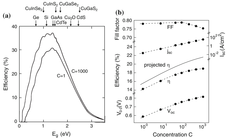
Fig. 22.55 (a) Ideal quantum efficiency of solar cells (single junction) as a function of band gap and light concentration C . The band gaps of some important semiconductors are denoted by arrows. Adapted from [1585]. (b) Properties of a silicon solar cell (water cooled) as a function of light concentration. Solid line is theoretically projected efficiency, dashed lines are guides to the eye. Adapted from [500]
