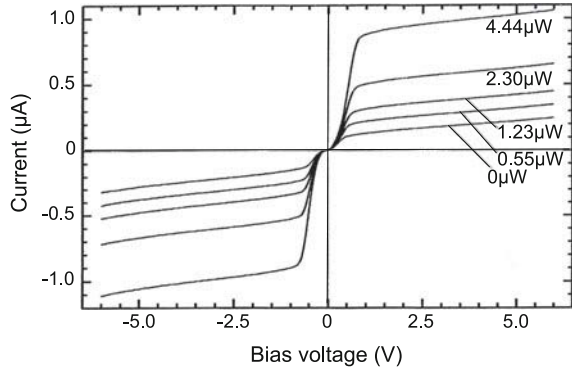
Fig. 22.25 dc I - V characteristic of an InGaAs/InP MSM photodetector (InP:Fe/InGaAs:Fe/InP:Fe, finger separation 1\text{ }\mu\text{m} , \lambda = 1.3\text{ }\mu\text{m} ) under illumination for dark environment ( 0\text{ }\mu\text{W} ) and various illumination levels as labeled. Adapted from [1552]
