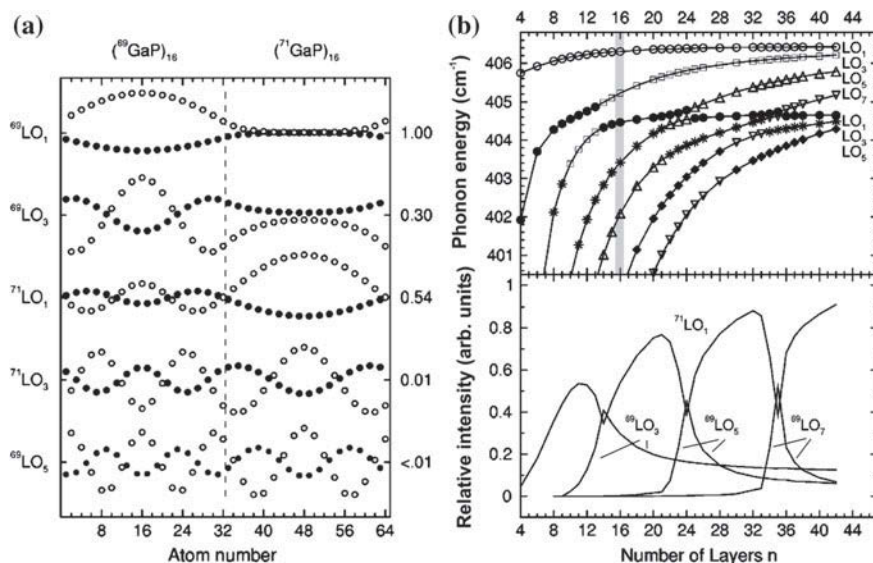
Fig. 12.44 (a) Atomic displacements [Ga ( filled dots ) and P ( open circles )] of odd-index LO modes in a ^{69}\text{Ga}_{16}\text{P}/^{71}\text{Ga}_{16}\text{P} superlattice unit cell. These modes have even parity with respect to midlayer planes, which are at atom numbers 16 and 48 in this example. The labels on the right identify the predominant character of the mode, those on the left give the relative Raman intensities with respect to that of the ^{69}\text{LO}_1 mode. The tick marks on the vertical axis indicate zero displacement of the respective mode. (b) Upper panel : Energies and characters of odd-index LO phonon modes in GaP isotope SLs as calculated within the planar bond charge model for the case of ideal interfaces. ^{69}\text{LO}_m modes are shown as open symbols ; ^{71}\text{LO}_m modes as full symbols . The shaded area marks n = 16 for which the atomic displacements of the modes are shown in part (a). Lower panel : Calculated intensities of the modes relative to that of the ^{69}\text{LO}_1 phonon mode. Adapted from [335], reprinted with permission, © 1999 APS
