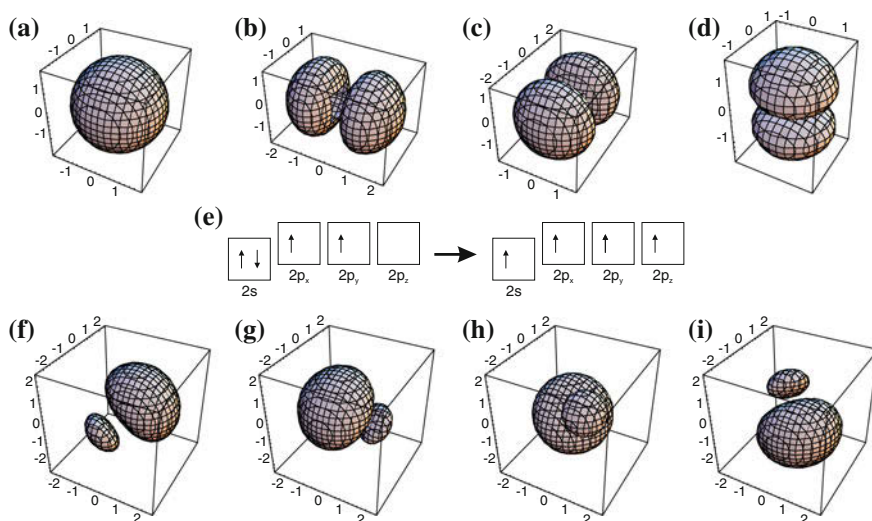
Fig. 2.3 (a) s orbital, (b, c, d) p x , p y and p z orbital, (e) hybridization, (f, g, h, i) orbitals of the sp 3 hybridization: (f) (s + p_x + p_y + p_z)/2 , (g) (s + p_x - p_y - p_z)/2 , (h) (s - p_x + p_y - p_z)/2 , (i) (s - p_x - p_y + p_z)/2
