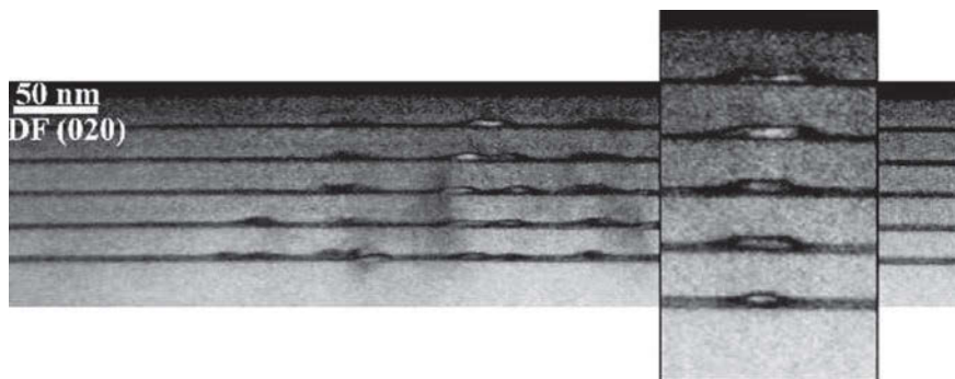
Fig. 14.27 Cross-sectional TEM image of a stack of five layers of quantum dots. Due to strain effects, vertical arrangement is achieved
