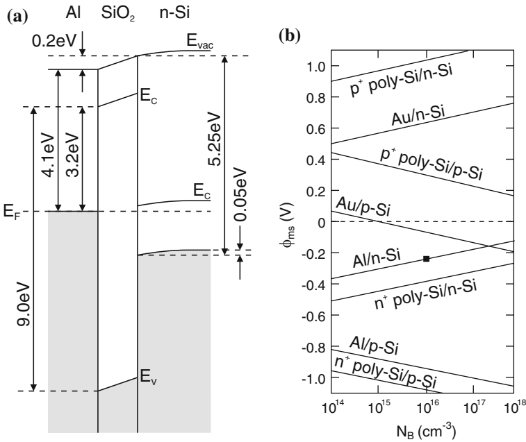
Fig. 21.36 (a) Schematic band diagram of an Al–SiO 2 –Si (n-type) diode with 50 nm oxide thickness and N_D = 10^{16} cm −3 for zero bias. Based on data from [1475]. (b) Difference of work functions \phi_{ms} for SiO 2 –Si MIS diodes and various doping levels and electrode materials (Al, Au and polycrystalline Si). The square represents the situation depicted in panel (a). Based on data from [1476]
