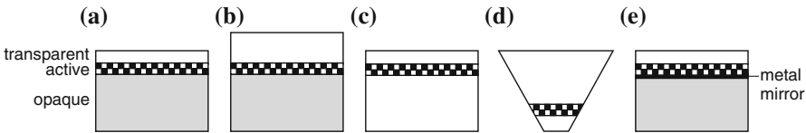
Fig. 23.8 (a) Standard LED layer sequence with opaque substrate (grey), active layer (checked) and transparent top, (b) thick window design with thick top layer (50–70 μm). (c) Transparent substrate (by rebonding, see Fig. 23.9), (d) chip shaping (cf. also Fig. 23.11). (e) Thin-film LED with metal mirror (black) and rebonding (cf. also Fig. 23.12)
