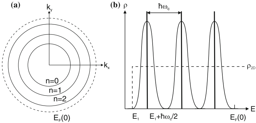
Fig. 13.12 2D electron gas in an external magnetic field. (a) Allowed states in k -space. (b) Density of states (DOS) \rho versus energy. Dashed line is two-dimensional DOS without magnetic field. Thick vertical lines : \delta -like DOS without broadening, curves : broadened DOS. Based on [991]
