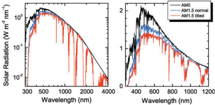
Fig. 22.50 Solar spectra (power per area and wavelength interval) for AM0 ( black line , extraterrestrial irradiance) and AM1.5 (sun at 41.8^\circ elevation above horizon) for direct normal irradiance ( blue line ) and global total irradiance ( red line ) on a sun facing surface (tilted 37^\circ towards the equator). Left (right) graph in log–log (linear) scales
