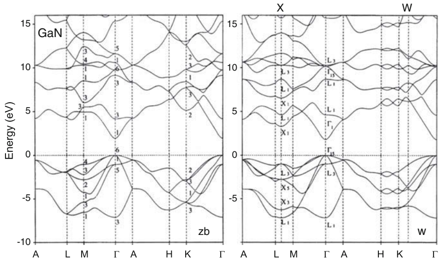
Fig. 6.8 Band structure of GaN (direct) in zincblende (zb) modification ( left ) and wurtzite (w) modification ( right ), both displayed in the wurtzite Brillouin zone to facilitate comparison
