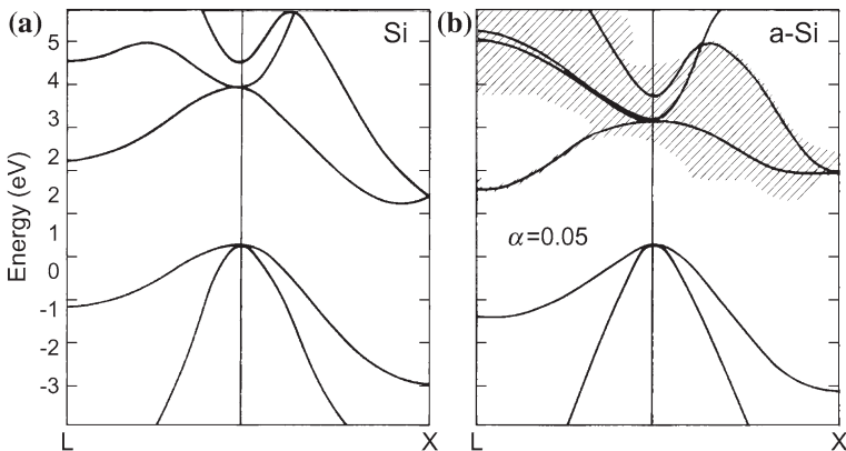
Fig. 6.22 (a) Calculated band structure of crystalline silicon. (b) Calculated band structure of amorphous silicon with \alpha = 0.05 (cf. (3.7)). The solid lines denote the real part of the energy, the shaded areas denote the regions with a width of twice the imaginary part of the energies centered around the real part. Adapted from [431]
