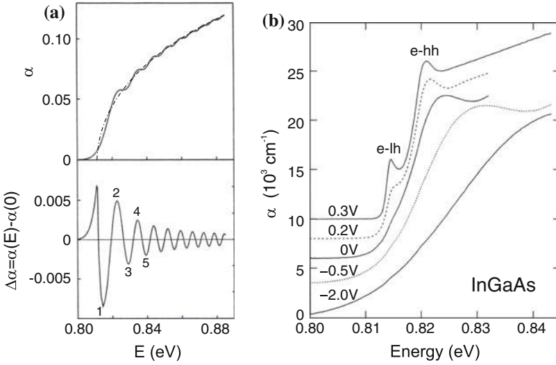
Fig. 13.3 (a) Theoretical absorption ( top panel ) with ( solid line ) and without ( dash-dotted line ) electric field for a volume semiconductor (without Coulomb interaction) and theoretical change of absorption ( bottom panel ). (b) Experimental absorption spectra of InGaAs on InP at T = 15 \text{ K} for various applied voltages as labeled. Adapted from [1081]
