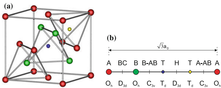
Fig. 3.18 (a) Unit cell of the zincblende structure with the indication of tetragonal symmetries. The position of the small yellow (blue) sphere is the tetrahedrally configured unoccupied positions of the A (B) sublattice, denoted with ‘T’ in part (b). (b) Line along [111] in the zincblende structure. The positions of the A and B atoms are denoted by red and green circles as labeled. Other positions are called the bond center (‘BC’), antibonding (‘AB’) relative to A and B atoms (‘A–AB’, ‘B–AB’), hexagonal (‘H’) and tetrahedral position (‘T’, blue and yellow circles)
