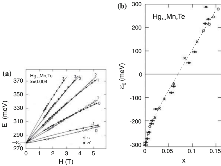
Fig. 16.3 (a) Energies of \Gamma_6 \rightarrow \Gamma_8 transitions versus magnetic field for \text{Hg}_{0.996}\text{Mn}_{0.004}\text{Te} at T = 2 K. Symbols are experimental values for two polarization directions as indicated. Numbers denote quantum numbers of transitions. Solid lines are theoretical fits. (b) Interaction gap versus Mn concentration for \text{Hg}_{1-x}\text{Mn}_x\text{Te} at T = 4.2 K. Various symbols represent data from different authors and methods. Dashed line is a guide to the eye. Adapted from [1229]
