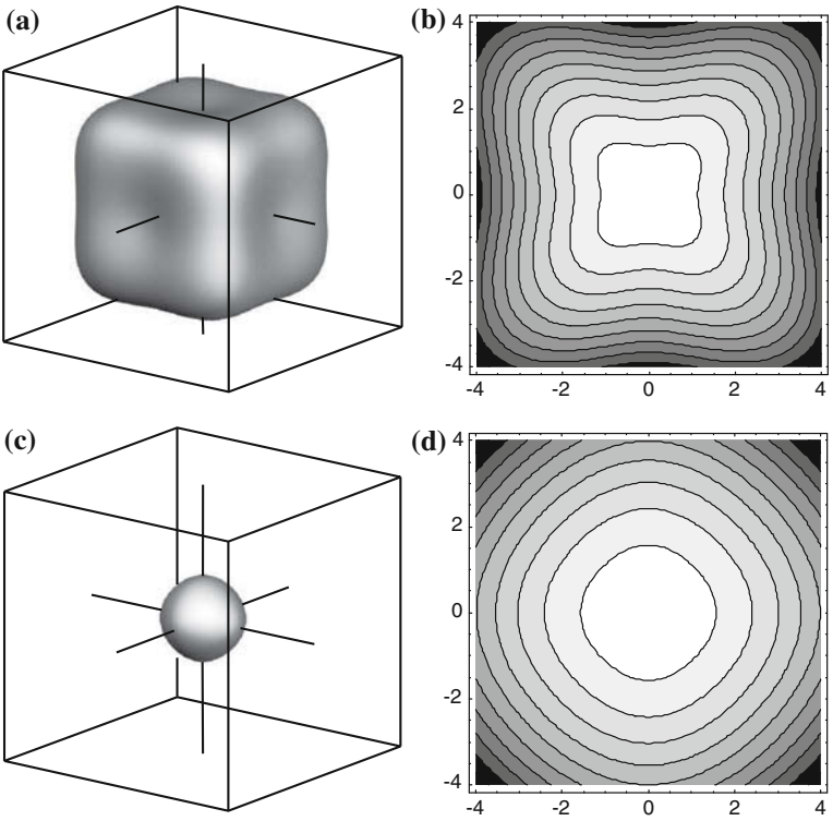
Fig. 6.35 Dispersion at the valence band edge of GaAs for (a, b) heavy holes and (c, d) light holes. (a, c) Constant energy surfaces and (b, d) isolines in the (k_x, k_y) -plane ( (b) and (d) have different energy scales)
