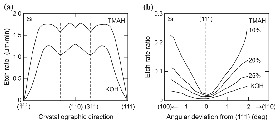
Fig. 4.21 (a) Etch rate of silicon for tetramethyl-ammonium-hydroxide (TMAH) water solution (25%) at 86^\circ\text{C} and 40% KOH at 70^\circ\text{C} as a function of crystallographic direction. (b) Detail of the anisotropy around the (111) direction for TMAH solutions with three different concentrations and 40% KOH, all at 86^\circ\text{C} . Adapted from [291]
