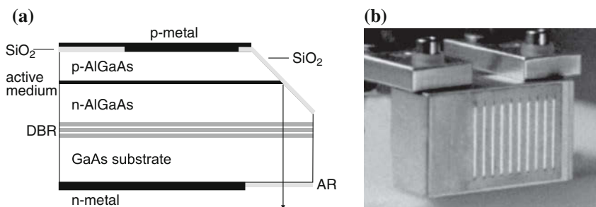
Fig. 23.64 (a) Principle of a surface-emitting laser. Light generated in the active region is internally reflected by the 45^\circ angled mirror and directed through the substrate; 'AR': antireflection coating, 'DBR': epitaxial Bragg mirror. (b) Light emission from a 10 \times 22 surface-emitting diode array. The light emission appears as stripes due to the broad beam divergence in the vertical direction. Part (b) reprinted with permission from [1716]
