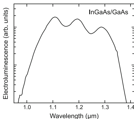
Fig. 23.25 Electroluminescence spectrum of a quantum dot LED designed for broad spectral range (at 5 \text{ kA/cm}^2 ). Adapted from [1669]
