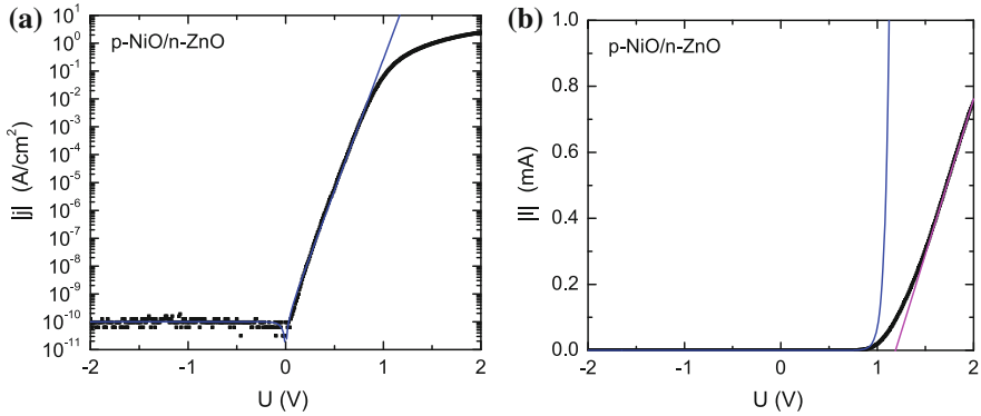
Fig. 21.50 (a) j - V -characteristic of NiO/ZnO bipolar diode (cmp. Sect. 21.4.6) in half-logarithmic plot. The blue line is a fit with ideality factor n = 1.8 . (b) I - V -characteristic in linear plot. The purple line in (b) is a linear fit (with R_s = 1.06 \text{ k}\Omega ) for the range where the series resistance dominates
