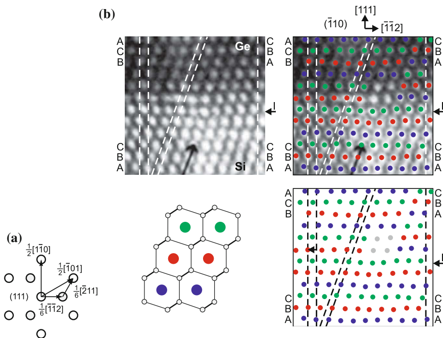
Fig. 4.19 (a) Graphical representation of the dislocation reaction of (4.22). (b) TEM image of the interface of a Ge/Si heterostructure with a [\bar{2}11]/6 Shockley partial dislocation. The image is overlaid with empty rod positions (as schematically shown in the lower left part of the figure) colored according to the stacking position (A: blue, B: red, C: green). The arrows labeled 'I' denote the position of the interface. Based on [289]
