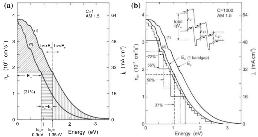
Fig. 22.54 (a) Number of photons n_{ph} per area and time in the sun spectrum (AM1.5, C = 1 sun) with an energy larger than a cutoff energy (curve 1) and graphical method to determine the quantum efficiency (from curve 2). Adapted from [1585]. (b) Number of photons in concentrated solar spectrum (AM1.5, C = 1000 sun) with an energy larger than a given energy and graphical method to determine the quantum efficiency of multi-junction solar cells. Adapted from [500] after [1585]
