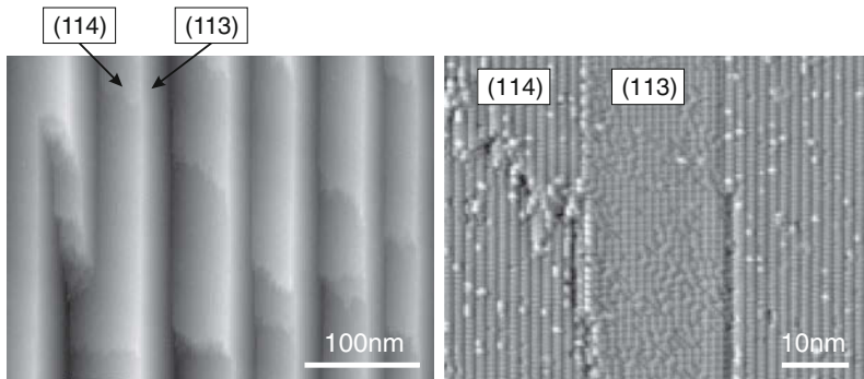
Fig. 11.9 STM images of a silicon surface close to (113), 21.5^\circ from (001) towards (111), i.e. (113)- 3.7^\circ . Adapted from [943]
