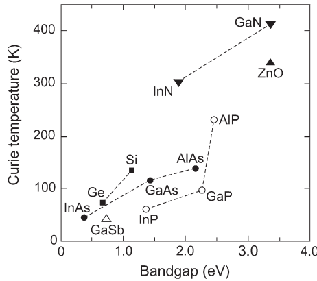
Fig. 16.5 Computed values of the Curie temperature T_C for various p-type semiconductors plotted versus the band gap ( dashed lines are guides to the eye). All materials contain 5 % Mn on the cation sublattice and a hole concentration of p = 3.5 \times 10^{20} \text{ cm}^{-3} . Values for T_C taken from [1233]
