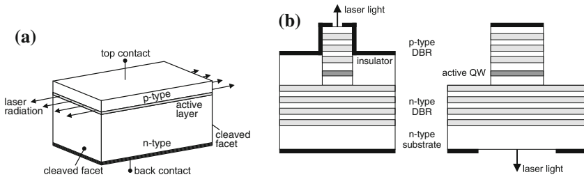
Fig. 23.29 (a) Schematic drawing of edge-emitting semiconductor laser. (b) Schematic drawings of vertical-cavity surface-emitting lasers with top emission (left) and emission through the substrate (right). Black areas are metal contacts
