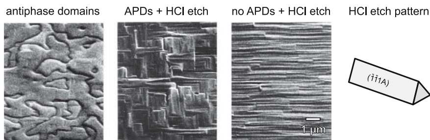
Fig. 4.36 Antiphase domains in InP on Si. HCl etches InP anisotropically and prepares (111)A planes. The etch patterns of layers with (without) APDs are cross-hatched (linear). Adapted from [324]
