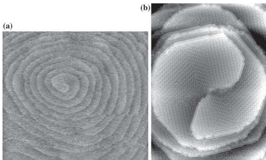
Fig. 4.16 (a) Atomic force microscopy image of growth spiral around a screw dislocation on a silicon surface; image width: 4\text{ }\mu\text{m} . (b) STM image (width: 75\text{ nm} ) of a screw-type dislocation with a Burgers vector of [000-1] on the N-face of GaN. The reconstruction is c(6 \times 12) . The c(6 \times 12) row directions correspond to \langle \bar{1}100 \rangle . Reprinted with permission from [287], © 1998 AVS
