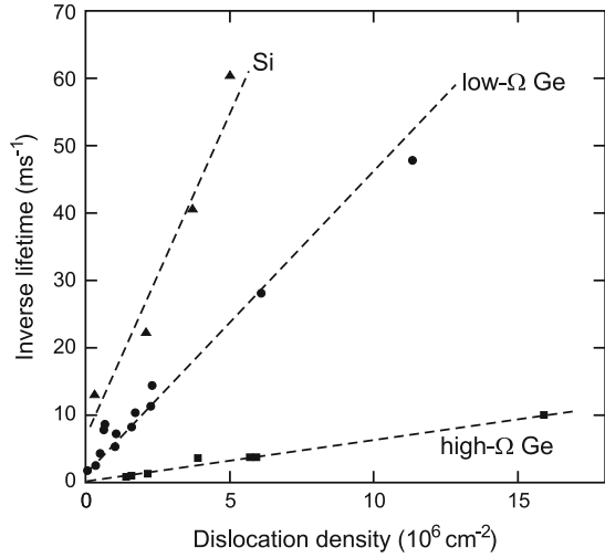
Fig. 10.34 Inverse minority carrier lifetime in n-type silicon ( 40\ \Omega\text{ cm} ), low resistivity Ge ( 3\text{--}5\ \Omega\text{ cm} ) and high resistivity Ge ( 30\text{--}40\ \Omega\text{ cm} ). Data from [918]
