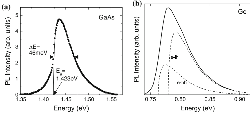
Fig. 10.2 (a) Photoluminescence spectrum of an undoped LPE-grown epitaxial GaAs layer at room temperature and low cw ( \lambda = 647 \text{ nm} ) excitation density ( 10 \text{ W/cm}^2 ). The solid line is a lineshape fit with (10.3) and E_g = 1.423 \text{ eV} and T = 293 \text{ K} . (b) Room temperature, direct ( e_f - h_f ) recombination from heavily n-doped ( 10^{19} \text{ cm}^{-3} ) germanium ( 1 \mu\text{m} thick Ge layer on silicon (001)) with biaxial (thermal) tensile strain. The strain-split valence band edge (Fig. 6.43) causes the e-hh and e-lh transitions (individual contributions with lineshape according to (10.3) shown as dashed lines) to occur at different energies. Adapted from [822]
