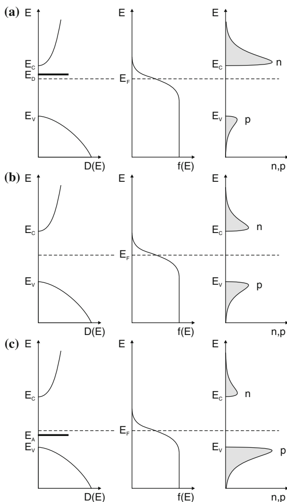
Fig. 7.4 Density of states (left column), Fermi distribution (center column) and carrier concentration (right column) for (a) n-type, (b) intrinsic and (c) p-type semiconductors in thermal equilibrium
