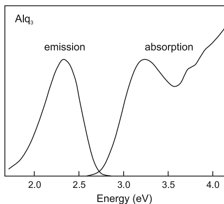
Fig. 17.10 Luminescence and absorption spectra of \text{Alq}_3 (vapor-deposited 150 nm thin film on a quartz substrate) at room temperature. Adapted from [1276]
