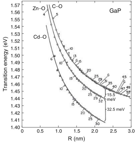
Fig. 10.24 Transition energies in GaP ( T = 1.6 K) of the donor–acceptor recombination involving the deep oxygen donor and C, Zn, and Cd acceptors, respectively. The lines follow (10.37) for E_{\text{g}}^{\text{GaP}} = 2.339 eV, \epsilon_r = 11.1 and (E_{\text{D}}^{\text{b}})_{\text{O}} = 893 meV, (E_{\text{A}}^{\text{b}})_{\text{C}} = 48.5 meV, (E_{\text{A}}^{\text{b}})_{\text{Zn}} = 64 meV, and (E_{\text{A}}^{\text{b}})_{\text{Cd}} = 96.5 meV. Predicted missing modes for GaP:C, O are labeled with ‘G’. Adapted from [886]
