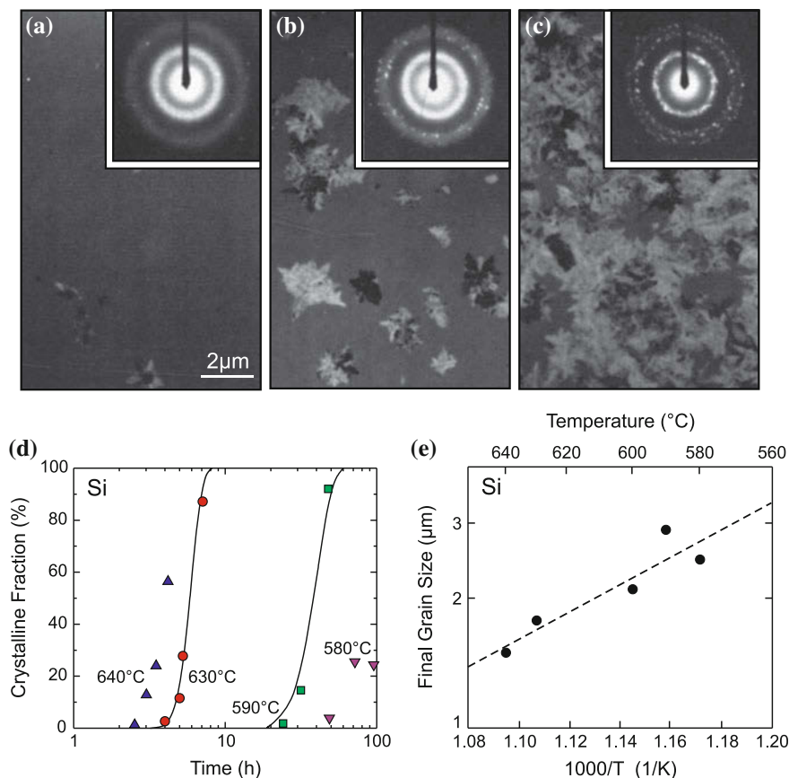
Fig. 24.51 Thermal annealing of 100 nm thick film of amorphous silicon (fabricated from LPCVD and amorphized by 100 keV \text{Si}^+ implantation with a dose of 5 \times 10^{15} \text{ cm}^{-2} ). TEM images and diffraction patterns ( insets ) for amorphized Si after (a) 4 h, (b) 5.25 h and (c) 7.1 h annealing at T = 630^\circ\text{C} . The crystalline fractions are 2, 28 and 87 %, respectively. (d) Crystalline fraction as a function of annealing time for various annealing temperatures as labeled. Symbols are experimental data, solid lines depict theory considering grain nucleation and growth. (e) Final grain size for various annealing temperature. Dashed line is exponential with a slope of 0.6 eV. Adapted from [1819]
