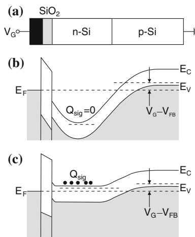
Fig. 22.43 (a) Schematic layers of MIS diode with buried-channel structure. Band diagram (b) after application of reverse voltage V_G and (c) with signal charge Q_{\text{sig}} . Adapted from [1569]
