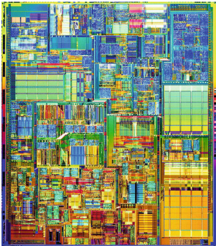
Fig. 24.30 The Intel TM Pentium 4 microprocessor (2000), circuit lines: 0.18\text{ }\mu\text{m} , 42 million transistors, clock speed: 1.5 GHz
