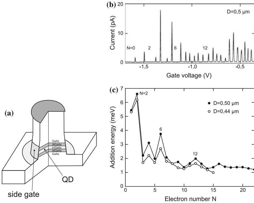
Fig. 14.19 (a) Schematic sample geometry for side-gated \text{In}_{0.05}\text{Ga}_{0.95}\text{As}/\text{Al}_{0.22}\text{Ga}_{0.68}\text{As} disk-shaped quantum dot. (b) Coulomb oscillations in the current versus gate voltage at B = 0\text{ T} observed for a D = 0.5 \mu\text{m} disk-shaped dot. (c) Addition energy versus electron number for two different dots with D = 0.50 and 0.44 \mu\text{m} . Adapted from [1161]
