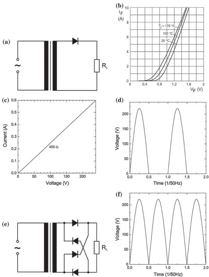
Fig. 21.61 (a) Single-path mains rectifier, (b) characteristics of Si diode (BYD127, Philips), (c) load characteristics of the mains rectifier ( R_L = 400\ \Omega ), (d) voltage output of single-path mains rectifier. (e) Depicts the schematic circuit of a bridge rectifier that works for both half-waves, (f) the resulting voltage output
