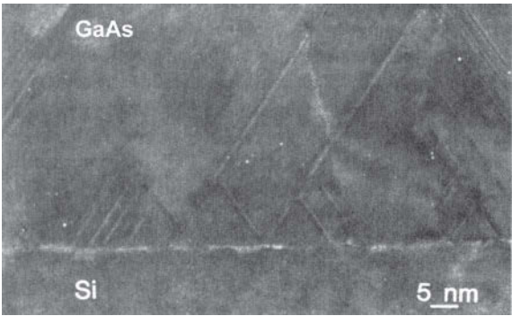
Fig. 4.27 Cross-sectional TEM image showing stacking faults in heteroepitaxial GaAs on Si. Adapted from [308]
