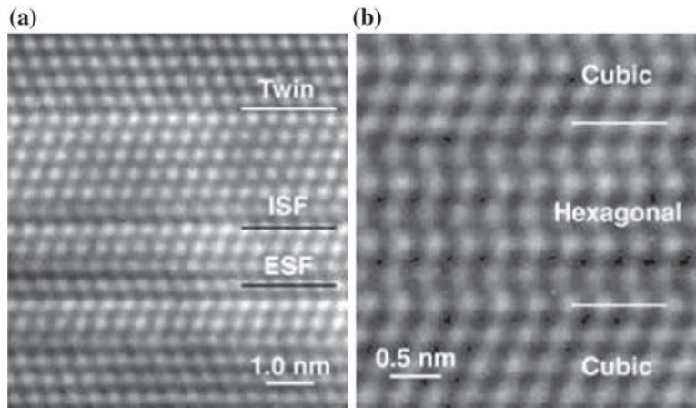
Fig. 4.26 HRTEM images of (a) thin-film silicon with intrinsic (labeled ‘ISF’) and extrinsic (‘ESF’) stacking faults and twin boundary (‘Twin’). (b) Six monolayer thick hexagonal (wurtzite) CdTe layer in cubic (zincblende) CdTe. Stacking order (from bottom to top) is: ABCABABABABC. . . Reprinted with permission from [307]
