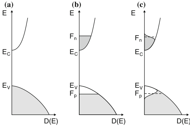
Fig. 23.33 Population (a) in thermodynamic equilibrium T = 0 K, (b) under inversion for T = 0 K, (c) under inversion for T > 0 K. Shaded areas are populated with electrons
