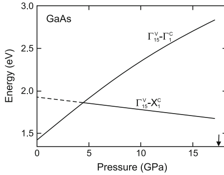
Fig. 6.42 Dependence of the direct \Gamma_{15}^V-\Gamma_1^C and indirect \Gamma_{15}^V-X_1^C band gap of GaAs ( T = 300 K) on pressure. Solid lines are interpolations of experimental data, dashed line is extrapolation to p = 0 . The crossing of the direct and indirect band gap occurs at 4.2 GPa. The arrow denotes the pressure of the phase transition from zincblende to an orthorhombic structure around 17 GPa. Adapted from [465]
