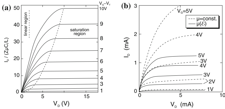
Fig. 24.23 (a) Idealized I – V characteristics for a MOSFET with constant mobility. The dashed line visualizes the drain (saturation) voltage for which the current is equal to I_{D,\text{sat}} . The solid lines are for various values of the gate voltage V_G - V_T = 1 – 10 V. Adapted from [500] (b) I – V characteristics taking into account the effect of field-dependent mobility ( solid lines ) in comparison to the constant-mobility model ( dashed lines ) for various gate voltages as labeled. Adapted from [1760]
