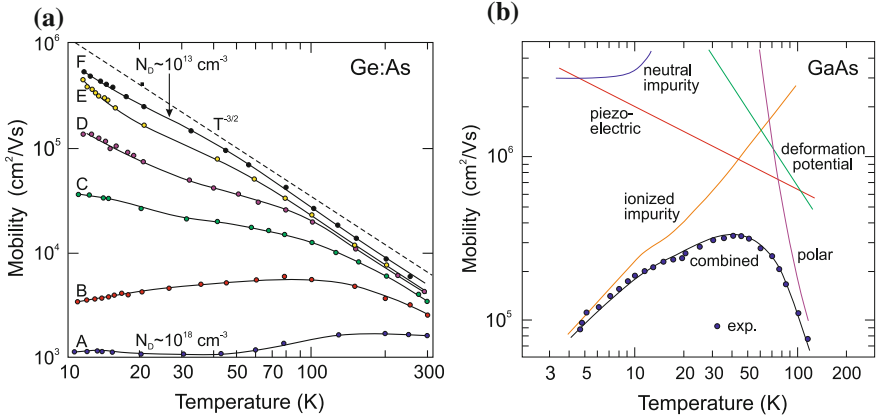
Fig. 8.4 (a) Temperature dependence of the electron mobility in n-doped Ge (for various doping levels from N_D \approx 10^{18} for sample A to 10^{13} \text{ cm}^{-3} for sample F in steps of a factor of ten). Dashed line indicates T^{-3/2} dependence of deformation potential scattering, solid lines are guides to the eye. Adapted from [515]. (b) \mu_n(T) for n-type GaAs ( N_D \approx 5 \times 10^{13} \text{ cm}^{-3} , N_A \approx 2 \times 10^{13} \text{ cm}^{-3} ). Solid lines are theoretical mobilities for various scattering mechanisms and combined mobility according to (8.12). Adapted from [654]
