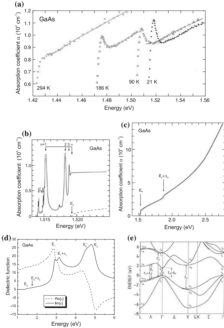
Fig. 9.8 (a) Absorption of GaAs close to the band gap at different temperatures. Adapted from [730]. (b) High-resolution absorption spectrum of highly pure GaAs at T = 1.2 \text{ K} in the exciton region. Dashed line is theory without excitonic correlation. Adapted from [731]. (c) Absorption spectrum of GaAs at T = 21 \text{ K} in the vicinity of the band gap. Adapted from [730]. (d) Complex dielectric function of GaAs at T = 300 \text{ K} , dashed (solid) line real (imaginary) part of dielectric constant. Peak labels relate to transitions shown in part (e). (e) Band structure of GaAs with band gap transition ( E_0 ) and higher transitions ( E_0 + \Delta_0 , E_1 , E_1 + \Delta_1 , E_2 , and E_2' ) indicated
