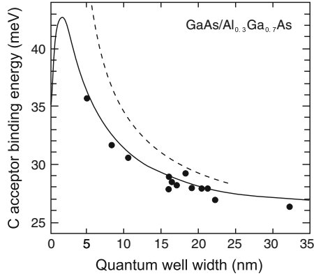
Fig. 12.30 Experimental values for the acceptor binding energy in GaAs/Al 0.3 Ga 0.7 As quantum wells (solid circles) from [1048] as a function of well width. Solid line is theory (variational calculation) for the well-center acceptor including top four valence bands and finite barriers, dashed line is hydrogen-like model with infinite barrier height. Adapted from [1049]
