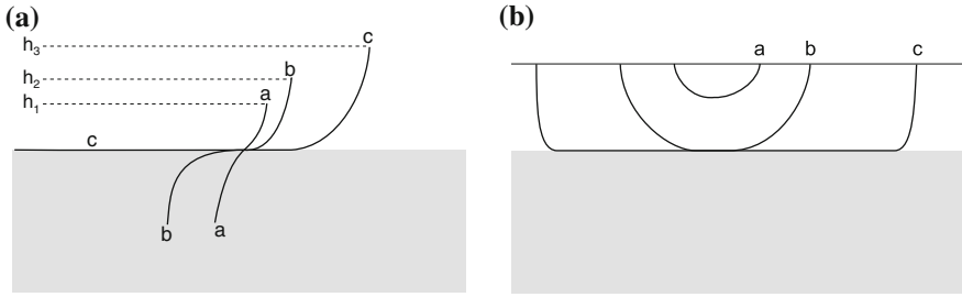
Fig. 5.35 Schematic formation of misfit dislocations by (a) elongation of a grown-in threading dislocation and (b) by the nucleation and growth of dislocation half-loops. (a) depicts a threading dislocation. Initially, for thickness h_1 the interface is coherent 'a', for larger thickness h_2 the interface is critical and the force of the interface on the dislocation is equal to the tension in the dislocation line, 'b'. For larger thickness, e.g. h_3 , the dislocation line is elongated in the plane of the interface, 'c'. In (b) 'a' denotes a subcritical dislocation half-loop, 'b' depicts a half-loop being stable under the misfit stress and for 'c' the loop has grown under the misfit stress into a misfit dislocation line along the interface
