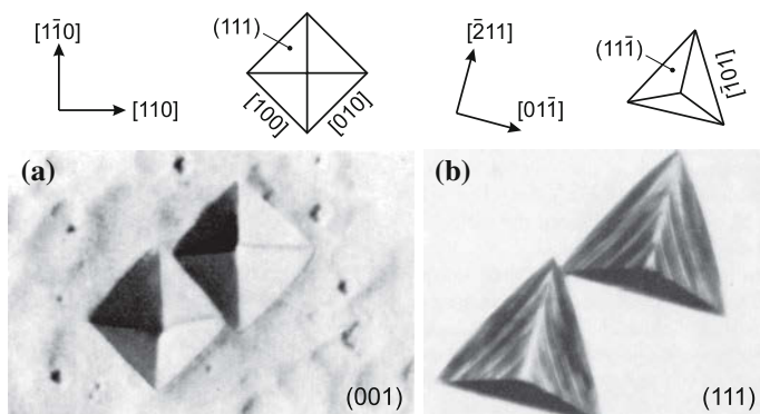
Fig. 4.22 Etch pits on germanium with (a) (001) and (b) (111) surface orientation. In both cases \{111\} facets are prepared by the etch. As etch in (b) a \text{HNO}_3/\text{HF}/\text{CH}_3\text{COOH} solution with \text{AgNO}_3 additive has been used. Width of the triangular etch pits is about 100\mu\text{m} . Adapted from [296]
