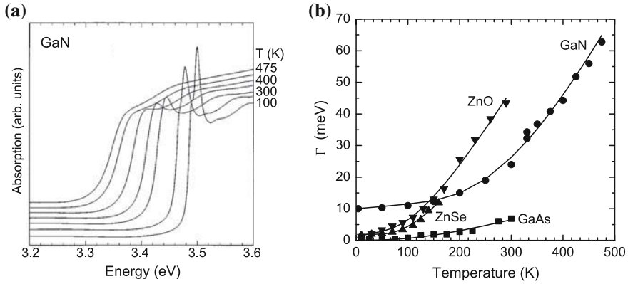
Fig. 9.21 (a) Absorption spectra of GaN bulk (0.38 μm thick epilayer on sapphire) for various temperatures T = 100, 200, 300, 350, 400, 450, and 475 K. Adapted from [756]. (b) Homogeneous broadening as a function of temperature, symbols are experimental data, solid lines are fits, cf. Table 9.5
