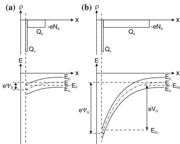
Fig. 24.21 Charge-carrier distribution ( top ) and band diagram ( bottom ) at the inverted p-region of a MOSFET for (a) thermodynamic equilibrium ( V_D = 0 ) and (b) nonequilibrium at drain
