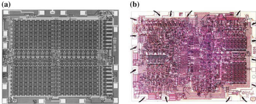
Fig. 24.29 (a) Intel TM 1103 1 KByte (1024 memory cells) dynamic random access memory (RAM), arranged in four grids with 32 rows and columns (1970), chip size: 2.9 \times 3.5 \text{ mm}^2 . (b) Intel TM 4004 microprocessor (1971), chip size: 2.8 \times 3.8 \text{ mm}^2 , circuit lines: 10 \mu\text{m} , 2,300 MOS transistors, clock speed: 108 kHz
