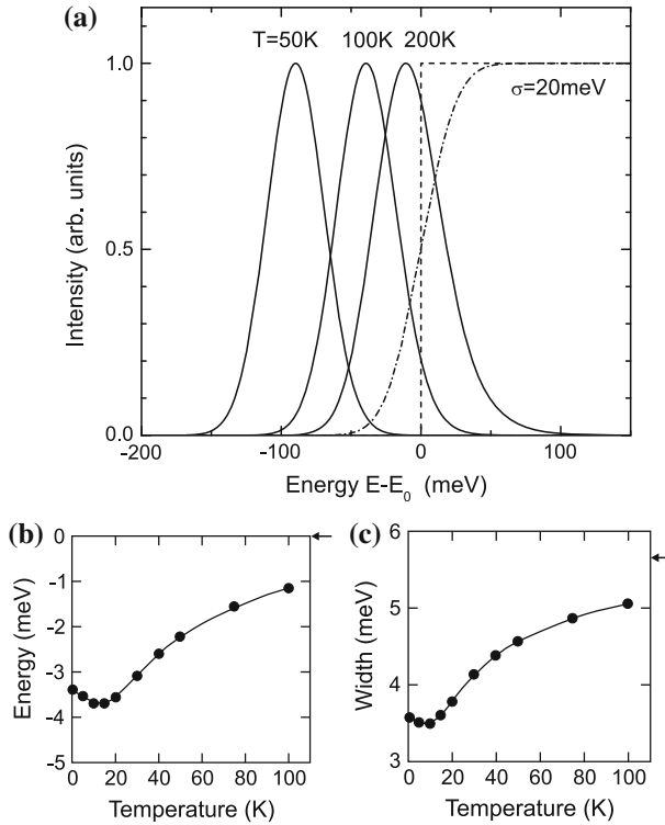
Fig. 12.40 (a) Recombination spectra ( solid lines , scaled to same height) of a model quantum well for different temperatures as labeled and complete thermalization, dashed ( dash-dotted ) line is unperturbed (inhomogeneously broadened by \sigma = 20\text{ meV} ) shape of the QW absorption edge. The energy scale is relative to the energy position of the unperturbed QW absorption edge at E_0 . (b) Theoretical energy position and (c) linewidth of exciton recombination from a model disordered quantum well. The high-temperature limits are marked by arrows . Parts (b, c) adapted from [1063]
