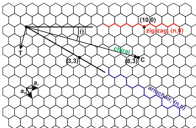
Fig. 18.1 Schematic atomic arrangement in graphene; the C–C bond length is d_{\text{C-C}} = 0.142 nm. Several vectors for making carbon nanotubes (cf. Sect. 18.2) are shown
