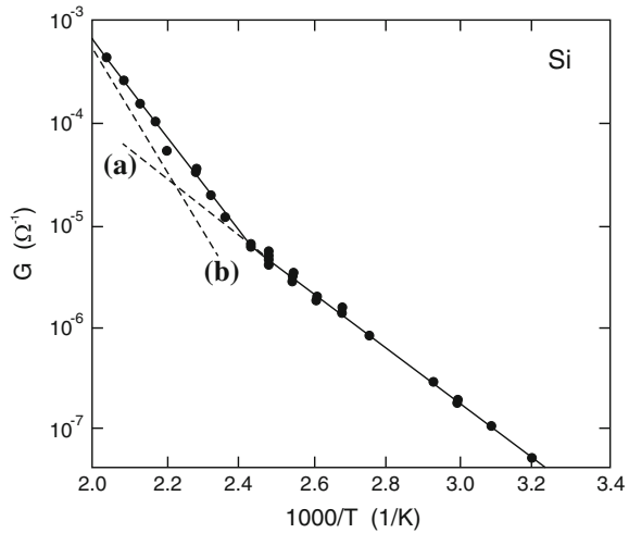
Fig. 22.37 Conductivity of a n-Si/SiO 2 -diode as a function of temperature ( 1/T ). The slope of the dashed lines is (a) \sim 0.56 eV ( \approx E_g/2 ) and (b) \sim 1.17 eV ( \approx E_g ). Adapted from [1564]
