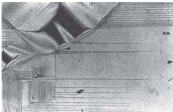
Fig. 15.9 Ferroelectric domains in a BaTiO 3 single crystal visualized by birefringence contrast. Reprinted with permission from [1200], © 1949 APS
