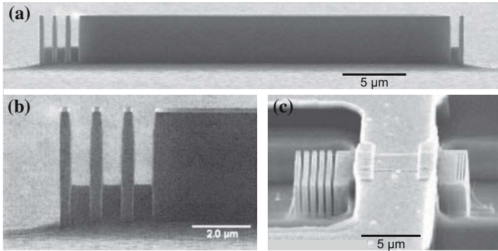
Fig. 23.44 SEM image of (a) an InP microlaser with third-order Bragg mirrors, (b) magnified view of the front facet with three slabs, (c) a 12 \mu\text{m} long microlaser with five third-order mirrors on the rear side and three first-order mirrors on the front side with top contact. From [1688]; part (b) reprinted with permission from [1687], © 2001 AIP
