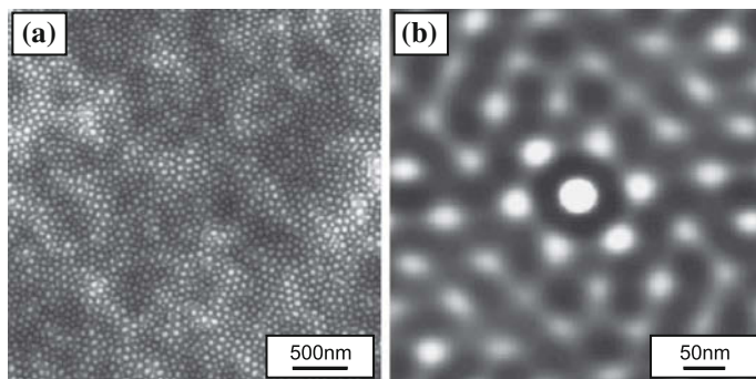
Fig. 14.31 (a) AFM image of a Si (001) substrate after 960 min of ion sputtering (1.2 keV Ar + , normal incidence). (b) Two-dimensional autocorrelation function from a 400 \times 400 \text{ nm}^2 area of image in part (a). Adapted from [1175]
