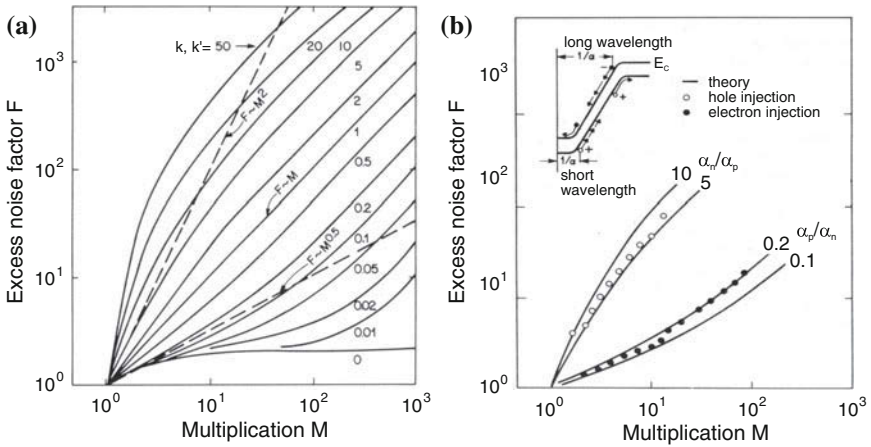
Fig. 22.29 (a) Excess noise factor for various values of the ratio of ionization coefficients k or k' . Adapted from [1554]. (b) Experimental results for F for a Si APD with 0.1 \mu\text{A} primary current. The empty (full) symbols are for short (long) wavelengths [primary hole (electron) current]. The inset shows the schematic band diagram of the np-diode under reverse bias. Adapted from [1555]
