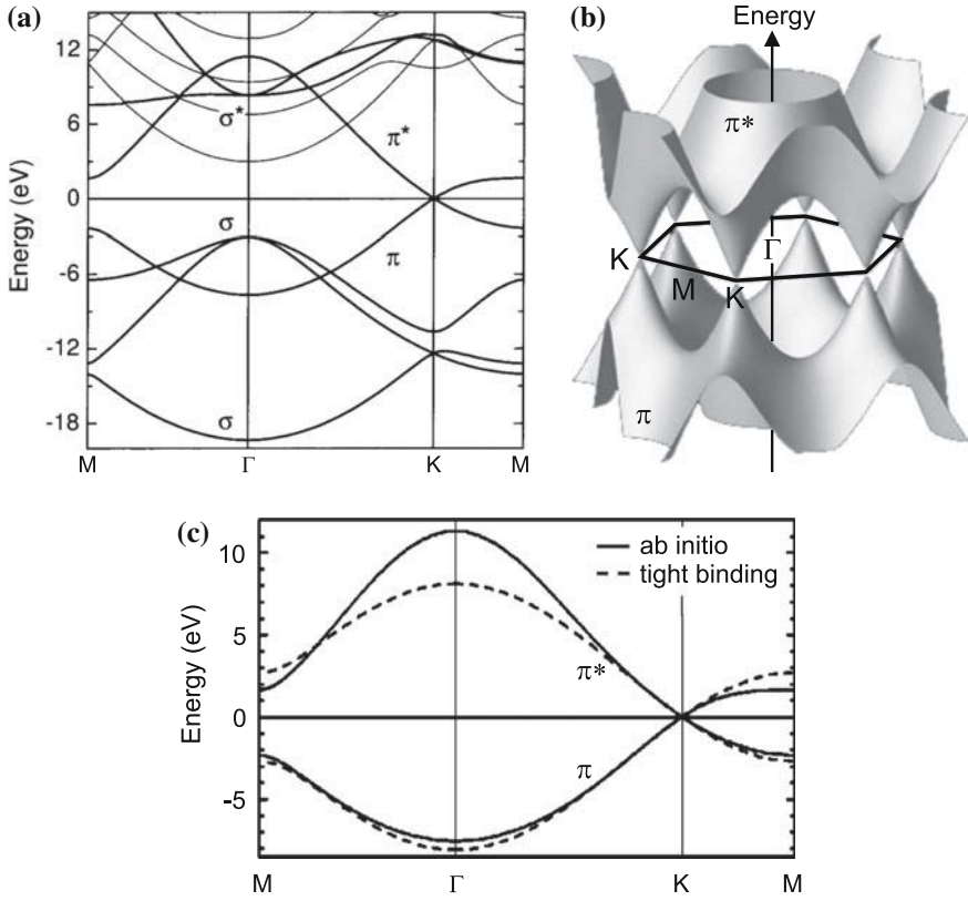
Fig. 18.4 (a) Band structure of graphene from first principles. (b) Three-dimensional representation E(k_x, k_y) of the \pi -bands of graphene. (c) Band structure of graphene with only \pi -bands shown, solid lines are ab-initio calculation, dashed lines are calculated with tight-binding approximation. Adapted from [1294]
