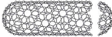
Fig. 18.12 A chiral nanotube (chiral vector is (10,5), \theta = -19.11^\circ ) with hemispherical caps at both ends based on an icosahedral C_{140} fullerene. The tube diameter is 1.036 nm. Adapted from [1311]
