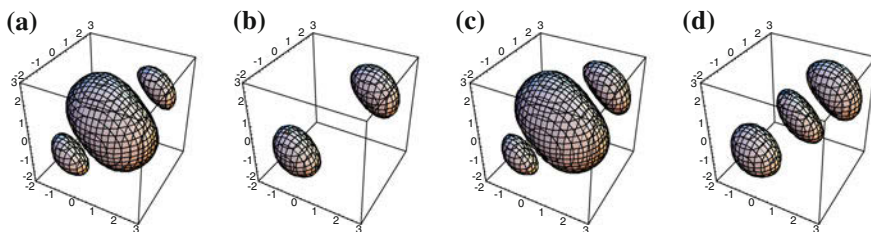
Fig. 2.7 Schematic representation of (a, c) bonding and (b, d) antibonding symmetric (a, b) and nonsymmetric (c, d) sp^3 orbitals
