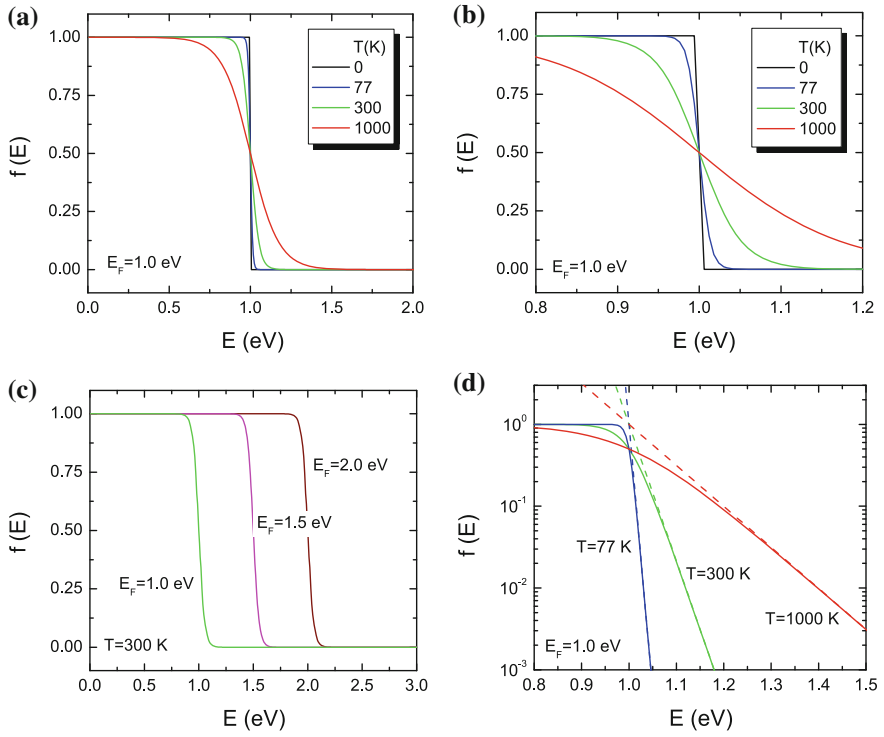
Fig. E.1 Fermi function for (a, b) different temperatures (for E_F = 1.0 eV) and (c) for different chemical potentials (for T = 300 K). (d) Fermi function ( solid lines ) compared with Boltzmann approximation ( dashed lines ) for various temperatures and E_F = 1.0 eV on semilogarithmic plot
