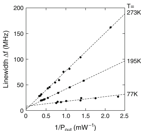
Fig. 23.63 Linewidth \Delta f of a cw GaAs/AlGaAs laser diode at various temperatures as a function of the inverse output power P_{\text{out}}^{-1} . At room temperature \alpha \approx 5 . Adapted from [1715]
