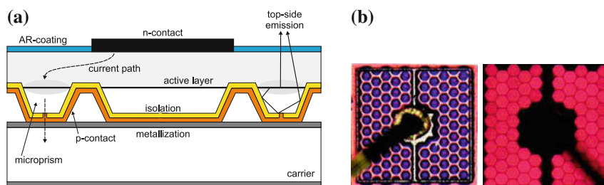
Fig. 23.12 (a) Scheme of thin-film flip-chip LED with microprisms. (b) image and luminescence image of thin film AlInGaP LED (chip length: 320\text{ }\mu\text{m} ). Reprinted with permission from [1650]
