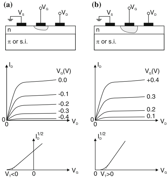
Fig. 24.16 Scheme (top), I_D versus V_D (center) and I_D^{1/2} versus V_G (bottom) I - V characteristics for (a) normally on (depletion) and (b) normally off (accumulation) n-type JFET. Adapted from [500]
