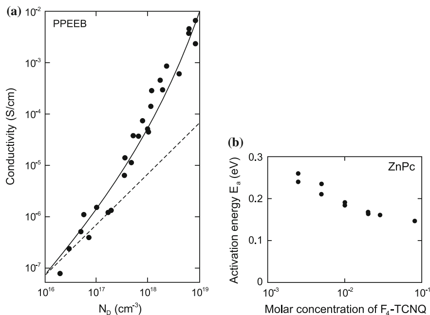
Fig. 17.7 (a) Conductivity (at 0.9 V/ \mu m) versus dopant concentration N_D for PPEEB films. Experimental data (circles) and fit (solid line) according to (17.1) with activation energy E_{a,0} = 0.23 eV and \beta = 6.5 \times 10^{-8} eV cm ( \mu = 0.2 cm 2 /Vs). Dashed line denotes linear relation between conductivity and N_D . Adapted from [1268]. (b) Thermal activation energy E_a of carriers (holes) in ZnPc:F 4 -TCNQ as a function of the molar dopant concentration. Adapted from [1265]
