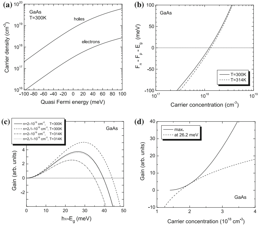
Fig. 23.34 Gain in the two-band model for GaAs. (a) Electron and hole concentrations at T = 300\text{K} as a function of the quasi-Fermi energies counted relative to the band edges, i.e. F_n - E_C and E_V - F_p . (b) Difference of quasi-Fermi levels as a function of carrier concentration ( n = p ) for GaAs at two different temperatures. (c) Gain spectra according to (23.12) for n = 2 \times 10^{18} and T = 300\text{K} (solid line), increased carrier density n = 2.1 \times 10^{18} and T = 300\text{K} (dashed line), higher temperature n = 2 \times 10^{18} and T = 314\text{K} (dash-dotted line) and same difference of the quasi-Fermi levels as for the solid line, n = 2.1 \times 10^{18} and T = 314\text{K} (dotted line). (d) Maximum gain (solid line) and gain at a particular energy (dashed line, for photon energy E_g + 26.2 \text{ meV} for which the gain is maximal for n = 2 \times 10^{18} and T = 300\text{K} , see solid line in part (c))
