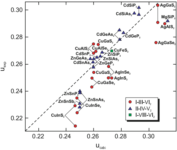
Fig. 3.22 Experimental values u_{\text{exp}} of the displacement parameter for various chalcopyrites versus the calculated value u_{\text{calc}} according to (3.10). The dashed line indicates u_{\text{exp}} = u_{\text{calc}} . Adapted from [191]
