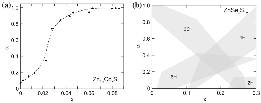
Fig. 3.30 (a) Hexagonality index \alpha (3.12) of \text{Zn}_{1-x}\text{Cd}_x\text{S} for various ternary compositions. Dashed line is a guide to the eye. (b) Regions of different polytypes in \text{ZnSe}_x\text{S}_{1-x} . Adapted from [211]
