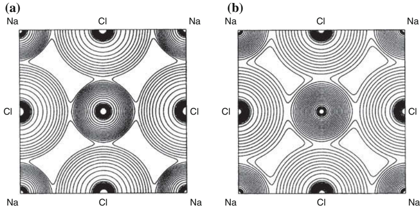
Fig. 2.12 (a) Experimental and (b) theoretical charge distribution in the (100) plane of NaCl. The lowest contour in the interstitial region corresponds to a charge density of 7\text{ e/nm}^3 and adjacent contours differ by \sqrt{2} . Differences are mainly due to the fact that the X-ray experiments have been made at room temperature. Adapted from [157]
