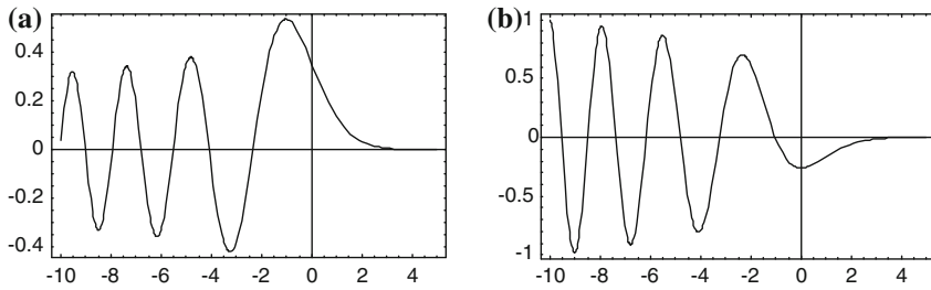
Fig. 13.2 (a) Airy function Ai(x) , (b) Ai'(x)
