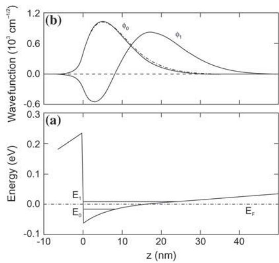
Fig. 12.35 (a) Conduction-band edge at a GaAs/ \text{Al}_{0.3}\text{Ga}_{0.7}\text{As} heterointerface ( T = 0 \text{ K} ) with two confined states at E_0 and E_1 marked with solid horizontal lines . In the GaAs channel there are 5 \times 10^{11} \text{ cm}^{-2} electrons. The barrier height is 300 meV, N_D^{\text{GaAs}} = 3 \times 10^{14} \text{ cm}^{-3} . The position of the Fermi level E_F is at E = 0 and indicated with a dash-dotted line . (b) Envelope wavefunctions \phi_0 and \phi_1 of the two confined states, dash-dotted line : calculation without exchange and correlation for state at E_0 . Adapted from [1055]
