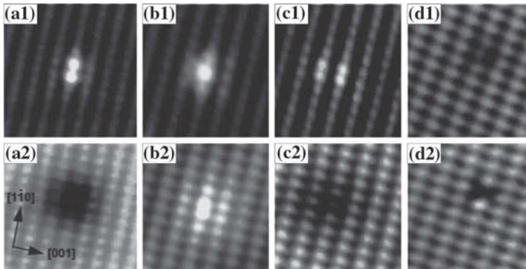
Fig. 4.1 Images of occupied ( upper frames ) and empty ( lower frames ) density of states of typical defects on Si-doped GaAs (110) surfaces. ( a1, a2 ) show a Ga vacancy, ( b1, b2 ) a \text{Si}_{\text{Ga}} donor, ( c1, c2 ) a \text{Si}_{\text{As}} acceptor and ( d1, d2 ) a \text{Si}_{\text{Ga}}\text{-V}_{\text{Ga}} complex. Adapted from [227]
