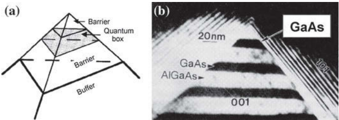
Fig. 14.23 (a) Schematic representation of growth on top of a predefined template, (b) cross-sectional TEM of quantum dot formation at the apex. Reprinted with permission from [1164], ©1992 MRS
