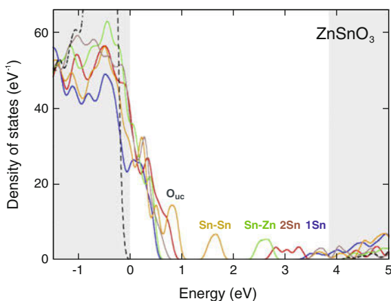
Fig. 6.49 Theoretical calculation for the density of states of crystalline ( dashed lines , conduction and valence bands indicated by gray areas ) and amorphous \text{ZnSnO}_3 with different configurations ( solid lines ). States due to under-coordinated oxygen ( O_{uc} ) and metal-metal binds are labelled. Adapted from [480]
