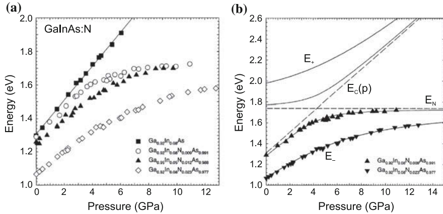
Fig. 6.41 (a) Dependence of the band gap of \text{Ga}_{0.92}\text{In}_{0.08}\text{As} alloy (squares) and nitrogen-doped (\text{Ga,In})\text{As} on (compressive) hydrostatic pressure, determined by photomodulated transmission at T = 295\text{ K} . (b) Pressure dependence of band gap for two (\text{Ga,In})(\text{As,N}) samples together with model calculation (6.58). The coupling parameter is V = 0.12\text{ eV} ( 0.4\text{ eV} ) for a nitrogen content of 0.9\% ( 2.3\% ). Adapted from [466]
