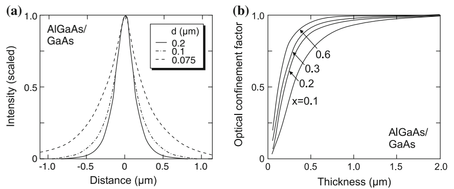
Fig. 23.38 (a) Optical mode (relative intensity) for various values of the thickness d of the active layer as labeled of a GaAs/ \text{Al}_{0.3}\text{Ga}_{0.7}\text{As} DHS laser, (b) Optical confinement factor \Gamma as a function of the thickness of the active layer and the Al concentration x of the barrier as labeled in a GaAs/ \text{Al}_x\text{Ga}_{1-x}\text{As} DHS laser. Adapted from [1674]
