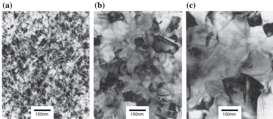
Fig. 3.13 Transmission electron micrographs of polycrystalline silicon (poly-Si). (a) As-deposited material from low-pressure chemical vapor deposition (LPCVD) at about 620 °C, grain size is about 30 nm. (b) After conventional processing (annealing at 1150 °C), average grain size is about 100 nm. (c) After annealing in HCl that provides enhanced point defect injection (and thus increased possibility to form larger grains), average grain size is about 250 nm. Adapted from [172]
