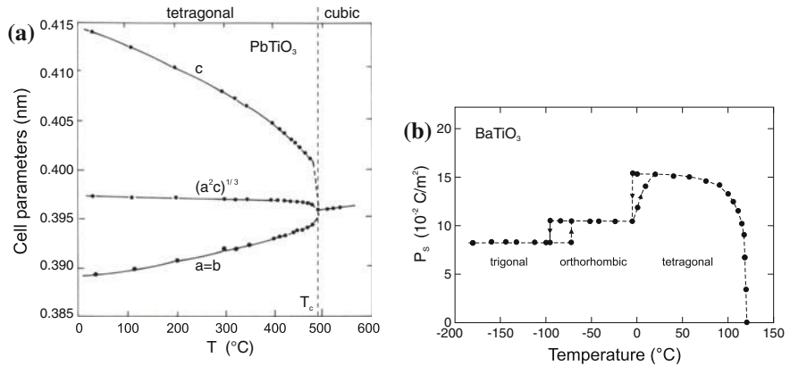
Fig. 15.4 (a) Cell parameters of PbTiO 3 as a function of temperature. Adapted from [1194]. (b) Phase transitions of BaTiO 3 as a function of temperature. The spontaneous polarization P_s points along \langle 100 \rangle , \langle 110 \rangle and \langle 111 \rangle in the tetragonal ( C_{4v} ), orthorhombic ( C_{2v} ) and trigonal ( C_{3v} , rhombohedral) phase, respectively. Adapted from [1195]
