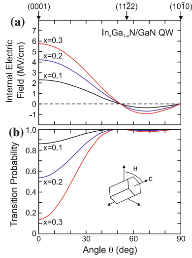
Fig. 15.14 (a) Internal electric field and (b) transition probability for electron-hole pairs in pseudomorphic \text{In}_x\text{Ga}_{1-x}\text{N}/\text{GaN} quantum well ( L_w = 3 \text{ nm} ) for three different indium contents x as labeled. \theta denotes the angle between the c -axis and the normal of the interface plane (see inset ). Based on [1213]
