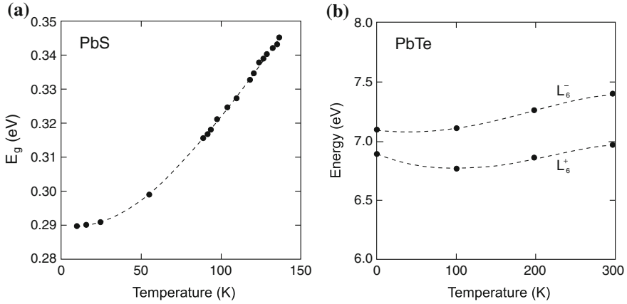
Fig. 6.24 (a) Band gap versus temperature for PbS. (b) Theoretical position of L_6^+ and L_6^- as a function of temperature for PbTe. Adapted from [410]
