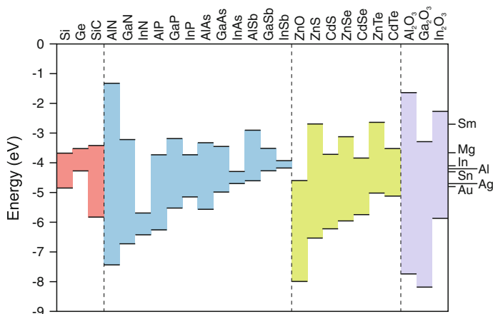
Fig. 12.21 Position of conduction and valence-band edges for a variety of semiconductors (relative to a common vacuum level at E = 0 eV). Based on values from [1032], for \text{Al}_2\text{O}_3 (on InP) from [1033], for \text{Ga}_2\text{O}_3 (on GaN) from [1034] for \text{In}_2\text{O}_3 (on Si) from [1035, 1036]. On the right hand side the work functions of several metals are shown for comparison.
