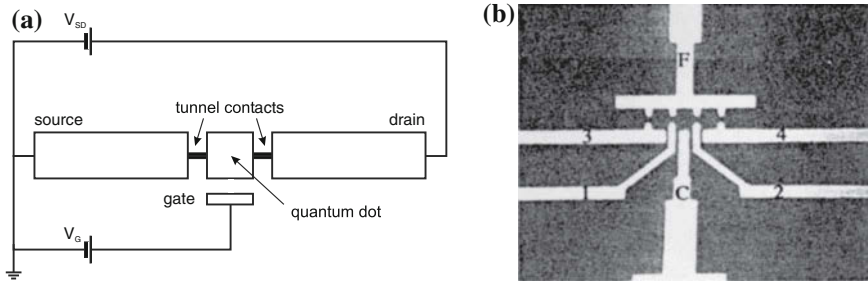
Fig. 14.16 (a) Schematic drawing of a quantum dot with tunnel contacts and gate electrode. (b) Realization with an in-plane gate structure. The distance between 'F' and 'C' (gate electrode) is 1\ \mu\text{m} . Electron transport occurs from a 2DEG between 3/F to 4/F through the quantum points contacts 1/3 and 2/4 . Part (b) reprinted with permission from [1160]
