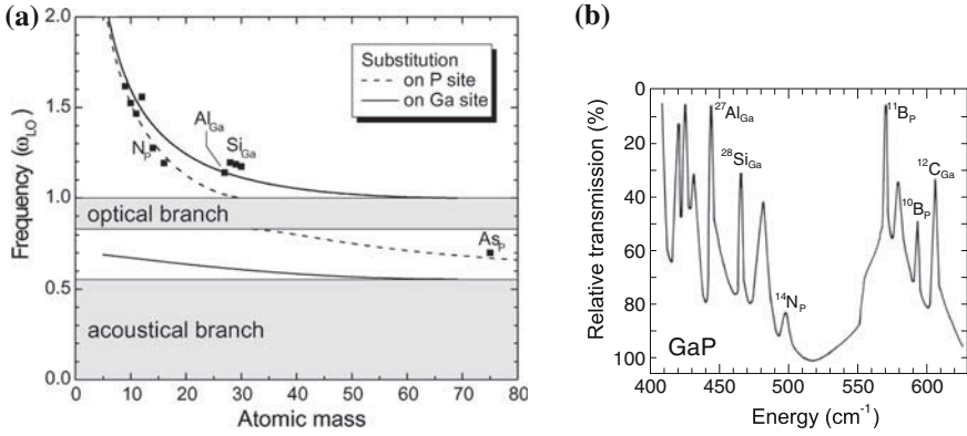
Fig. 5.14 (a) Numerical simulation of a linear chain model for GaP ( M_1 = 31 , M_2 = 70 ). Energy of local vibrational modes (dashed (solid) line): substitution on P (Ga) site in units of the optical phonon frequency at \Gamma ( \omega_m = 45.4 meV). The grey areas indicate the acoustic and optical phonon bands. Solid squares are experimental data (from [337]), scaled to the theoretical curve for the ^{27}\text{Al}_{\text{Ga}} LVM frequency. (b) Differential transmission spectrum of GaP structure (nitrogen-doped layer on zinc-doped compensated substrate) against pure crystal ( T = 77 K). Data from [342]
