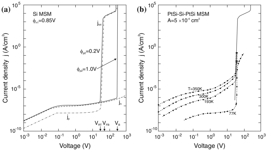
Fig. 22.23 Current–voltage characteristics of a Si MSM structure, N_D = 4 \times 10^{14} \text{ cm}^{-3} , L = 12 \mu\text{m} (thin, polished, (111)-oriented wafer), T = 300 \text{ K} . (a) Theory for two different values of \phi_{p2} , (b) experiment (for \phi_{p2} = 0.2 \text{ V} ). Adapted from [1551]
