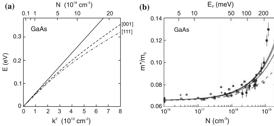
Fig. 6.31 (a) Dispersion relations for the conduction band of GaAs. The solid line is parabolic dispersion (constant effective mass). The dashed ( dash-dotted ) line denotes the dispersion for \mathbf{k} along [001] ([111]) from a five-level \mathbf{k} \cdot \mathbf{p} model (5LM). (b) Cyclotron resonance effective mass of electrons in GaAs as a function of the Fermi level ( upper abscissa) and the corresponding electron concentration ( lower abscissa). The dashed line is from a 2LM according to (6.43) with E_0^* = 1.52 eV. The solid lines are for a 5LM for the three principal directions of the magnetic field. The symbols represent experimental data from different sources. Data from [451]
