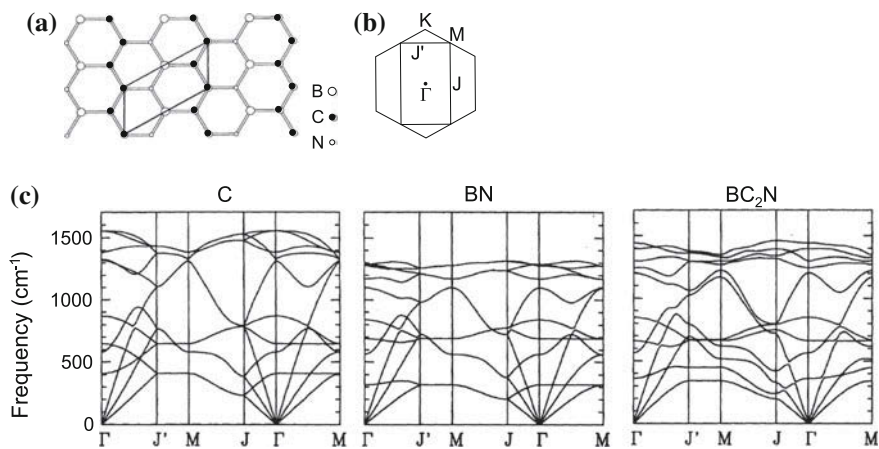
Fig. 18.9 (a) Crystal structure of BC_2N . (b) Brillouin zone of BC_2N (rectangle) and C, BN (hexagon). (c) Phonon dispersion of graphene (C) and BN- and BC_2N -sheets. Adapted from [1306]
