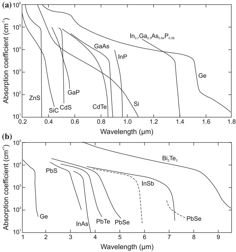
Fig. 22.13 Optical absorption coefficient of various semiconductor materials (as labeled) used for photodetectors (a) in the UV, visible and near-infrared range (at room temperature) and (b) in the mid-infrared spectral range at room temperature ( solid lines ) and at 77 K ( dashed lines ). Based on [1548]
