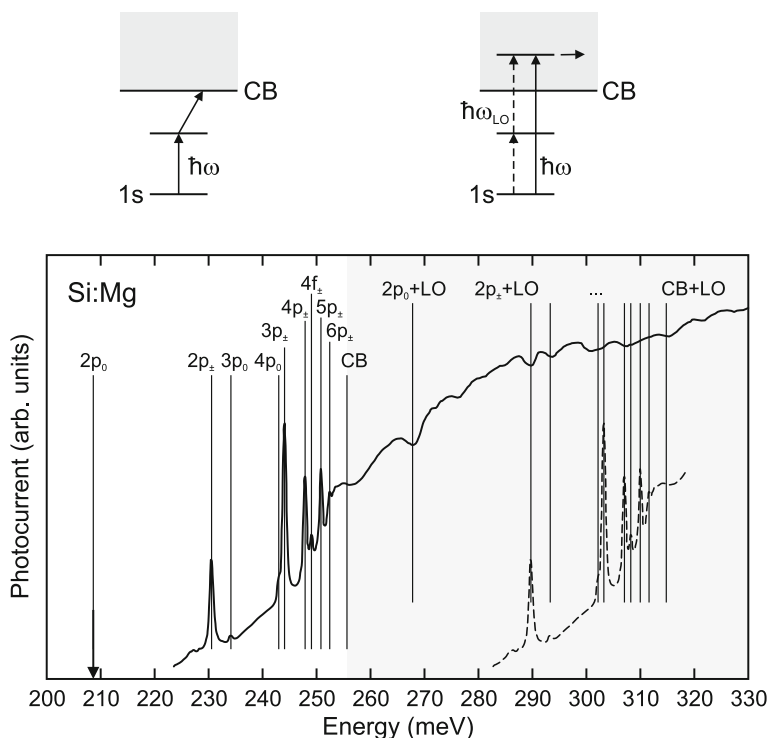
Fig. 9.34 Photocurrent spectrum of Si:Mg. Transitions are due to \text{Mg}_i^+ from its 1s state to excited states as labeled and indicated by vertical lines. CB denotes the conduction band edge (ionization limit). Above the CB edge (shaded area) phonon-assisted absorption occurs (Fano resonances). For comparison the absorption spectrum below CB is shown shifted by the phonon energy (dashed line). Above the plot, the transition mechanisms (photothermal ionization and Fano resonance) are schematically shown. Adapted from [795]
