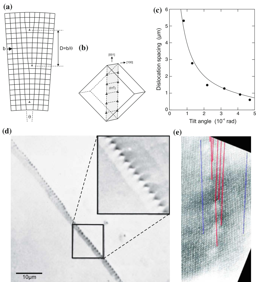
Fig. 4.31 (a) Scheme of a small-angle (pure tilt) grain boundary. (b) Model of edge dislocations in a \{110\} plane in Ge. (c) Relation of dislocation distance d and tilt angle \theta for various small-angle grain boundaries in Ge. Solid line is relation d = 4.0 \times 10^{-8}/\theta . (d) Optical image of an etched (CP-4 etch) Ge sample with a small-angle grain boundary. Adapted from [321]. (e) HRTEM image of a small-angle grain boundary in Si with dislocations highlighted. From [322]
