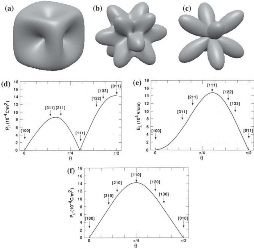
Fig. 15.12 Three-dimensional view of the (a) total, (b) longitudinal and (c) transverse polarization in uniaxially compressed GaAs. Adapted from [1203]. (d) Transverse polarization P_{\parallel} (parallel to the interface) and (e) longitudinal electric field E_{\perp} (perpendicular to the interface) in the InGaAs layer of a GaAs/In 0.2 Ga 0.8 As superlattice with joint in-plane lattice constant (obtained from energy minimization, 1.4 % lattice mismatch, the InGaAs is under compressive and the GaAs under tensile strain). The layer thicknesses of the GaAs and InGaAs layers are identical. The quantities are shown for various orientations of the growth direction. The vector of the growth direction varies in the (01–1) plane ( \phi = \pi/4 ) with polar angle \theta reaching from [100] ( 0^\circ ) over [111] to [011] ( 90^\circ ). Image (f) depicts the transverse polarization P_{\parallel} ( P_{\perp} = 0 in this geometry) for growth directions in the (001) plane ( \phi = 0 ). Parts (d, e, f) reprinted with permission from [1204], © 1988 AIP
