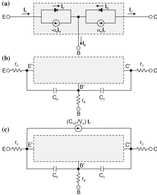
Fig. 24.7 Ebers–Moll model of a transistor, ‘E’: emitter, ‘C’: collector and ‘B’: base. Currents are shown for a pnp transistor. (a) Basic model (grey area in (b), (c)), (b) model with series resistances and depletion-layer capacitances, (c) model additionally including the Early effect ( V_A : Early voltage)
