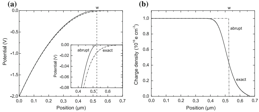
Fig. 21.7 (a) Potential \phi and (b) charge density \rho across the depletion layer of a Schottky n-GaAs diode. Calculation parameters are \epsilon_s = 12.5 \epsilon_0 , V_{bi} - V_{ext} = 2 \text{ V} (small reverse bias), N_D = 1 \times 10^{16} \text{ cm}^{-3} , T = 300 \text{ K} . Abrupt approximation is shown as solid lines , exact (numerical) calculation as dash-dotted line . Dashed line in (a) indicates depletion layer width w_0 in the abrupt approximation
