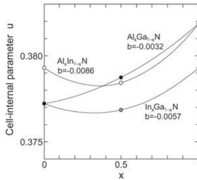
Fig. 3.41 Theoretical values ( T = 0\text{K} ) for the cell-internal parameter u as a function of the composition for group-III nitride alloys. The solid lines are quadratic curves (bowing parameter b is shown) through the points for x = 0, 0.5 , and 1.0 . Data from [224]
