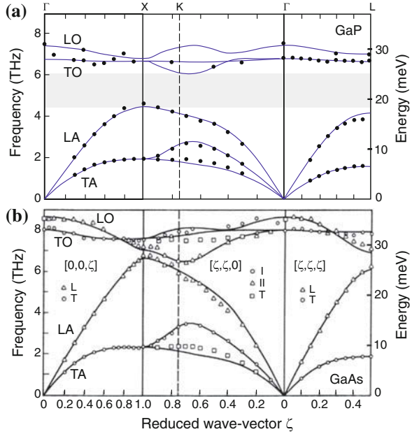
Fig. 5.6 Phonon dispersion in (a) GaP and (b) GaAs. Experimental data ( symbols ) and theory ( solid lines , 14-parameter shell model). 'L' and 'T' refer to longitudinal and transverse modes, respectively. 'I' and 'II' (along [\zeta, \zeta, 0] ) are modes whose polarization is in the (1, \bar{1}, 0) plane. The grey area in (a) denotes the gap between acoustical and optical states. (a) Adapted from [331], (b) adapted from [329]
