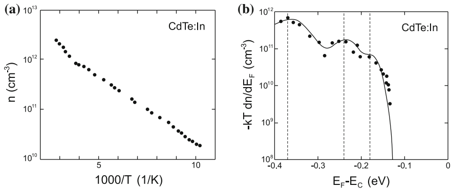
Fig. 7.20 (a) Electron concentration versus temperature as determined from Hall effect for a CdTe sample doped with indium. (b) -kT \, dn/dE_F , as determined from the experimental Hall data (symbols). The solid line is theory for three donor levels ( E_{D1} = E_C - 0.37\text{ eV} , N_{D1} = 2.5 \times 10^{12}\text{ cm}^{-3} ; E_{D2} = E_C - 0.24\text{ eV} , N_{D2} = 7.0 \times 10^{11}\text{ cm}^{-3} ; E_{D3} = E_C - 0.18\text{ eV} , N_{D3} = 2.5 \times 10^{11}\text{ cm}^{-3} ) whose energy positions are indicated by dashed lines. Adapted from [533]
