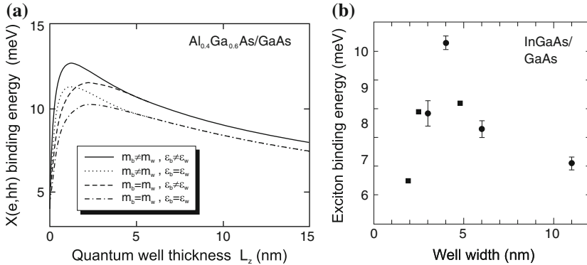
Fig. 12.31 (a) Theoretical (variational) calculation (solid line) of the heavy-hole exciton binding energy versus QW thickness in a GaAs/Al 0.4 Ga 0.6 As quantum well (using also different approximations, other lines). Adapted from [1050]. (b) Experimental exciton binding energy in In x Ga 1-x As/GaAs quantum wells of different thickness. Circles: data and error bars from [1051], x unspecified, squares: data from [1052], x = 0.18
