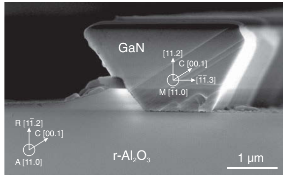
Fig. 12.16 SEM cross-sectional image of MOVPE GaN grown on patterned r-sapphire exposing a (11.2) growth front. Based on SEM image courtesy of F. Tendille
