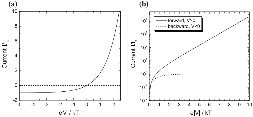
Fig. 21.13 Ideal diode I - V characteristics I = I_s (\exp(eV/kT) - 1) (a) in linear plot and (b) semilogarithmic plot
