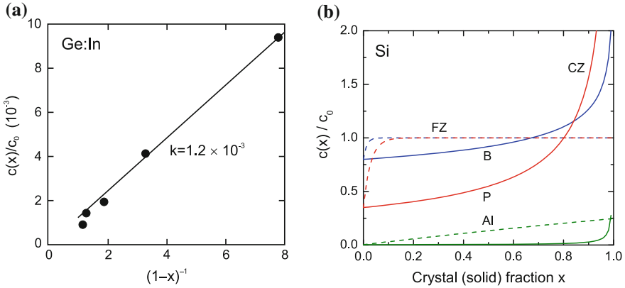
Fig. 4.6 (a) Relative concentration of indium along a CZ-grown germanium crystal. Absolute concentration is in the 10^{16} \text{ cm}^{-3} range. Solid line follows (4.19) with k = 1.2 \times 10^{-3} . Symbols are experimental data from [254]. (b) Impurity distribution (relative concentration c(x)/c_0 ) for CZ (solid lines) and FZ (4.20) (dashed lines, z = 0.01 ) silicon crystals for B (blue), P (red), and Al (green). Distribution coefficients have been taken from Table 4.2. Note crossing of B and P lines and possibly associated change from p-type to n-type (cmp. Fig. 1.7)
