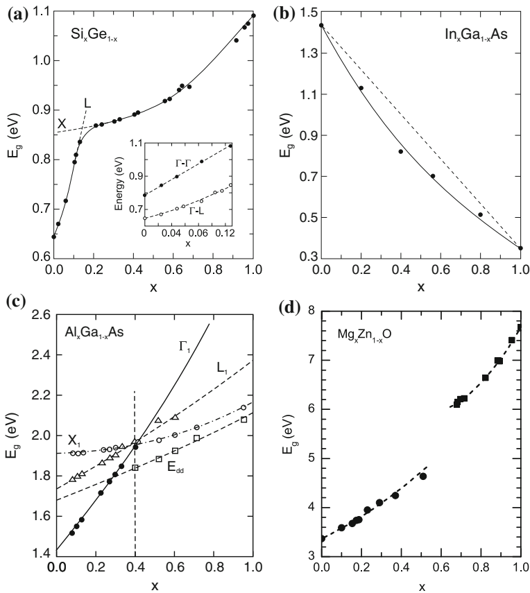
Fig. 6.19 (a) Band gap of \text{Si}_x\text{Ge}_{1-x} alloy ( T = 296\text{ K} ) with a change from the conduction-band minimum at L (Ge-rich) to X. The inset depicts the transition energy of the indirect ( \Gamma -L) and direct ( \Gamma - \Gamma ) absorption edge for low Si content. Adapted from [424]. (b) Band gap (at room temperature) of \text{In}_x\text{Ga}_{1-x}\text{As} . The solid line is an interpolation with bowing ( b = 0.6\text{ eV} ) and the dashed line is the linear interpolation. Data from [421]. (c) Band gap (at room temperature) in the ternary system \text{Al}_x\text{Ga}_{1-x}\text{As} . For x < 0.4 the alloy is a direct, for x > 0.4 an indirect, semiconductor. E_{dd} denotes the energy position of a deep donor (cf. Sect. 7.7.6). Adapted from [425]. (d) Band gap (at room temperature) in the ternary system \text{Mg}_x\text{Zn}_{1-x}\text{O} . Data (from spectroscopic ellipsometry [426, 427]) are for hexagonal wurtzite phase (circles), and Mg-rich cubic rocksalt phase (squares). Dashed lines are fits to data with a different bowing parameter for each phase
