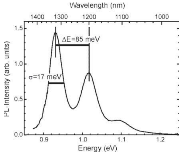
Fig. 14.36 Ensemble photoluminescence spectrum ( T = 293 K, excitation density 500 \text{ W/cm}^2 ) of InAs/GaAs QDs
