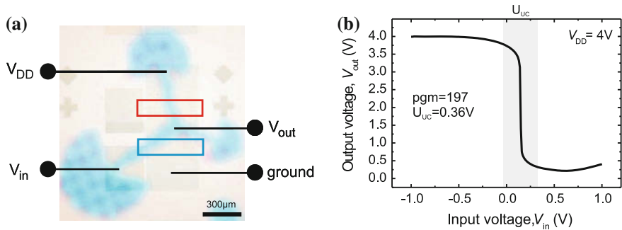
Fig. 24.54 (a) Optical image of transparent MESFET inverter based on ZnO. The two rectangles indicate the two gates. (b) Transfer characteristic for supply voltage V_{DD} = 4 V
