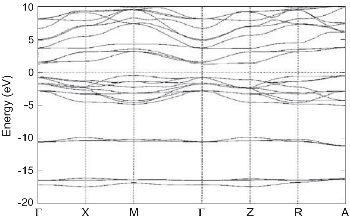
Fig. 6.15 Calculated energy band structure of BaTiO 3 along the major symmetry directions. The Fermi level ( E_F ) is set at zero energy. Adapted from [417]
