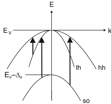
Fig. 9.43 Schematic optical transitions within the valence band
