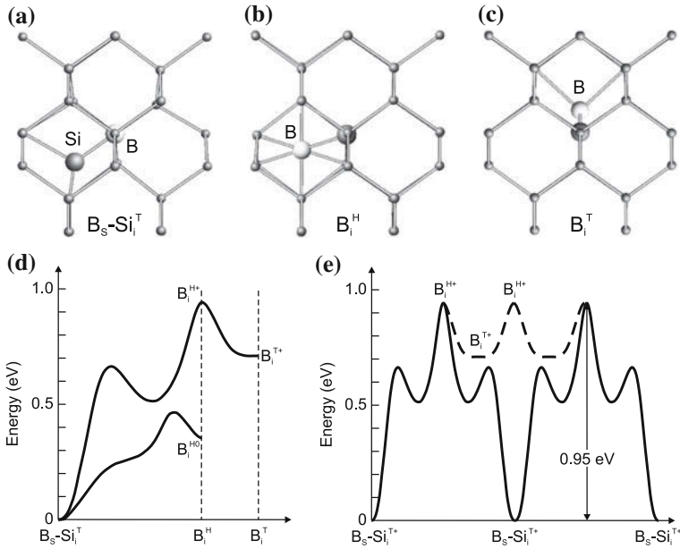
Fig. 4.5 Configurations of boron in Si: (a) Substitutional boron and Si self-interstitial at ‘T’ site ( B_S-Si_T^T ). Interstitial boron at (b) ‘H’ ( B_i^H ) and (c) ‘T’ site ( B_i^T ), each with the Si atoms on the Si lattice sites. The large bright ball represents the boron atom, large and small dark balls represent Si atoms. (d) Lowest energy barrier diffusion paths for positively charged and neutral B-Si states, total energy versus configuration. (e) Two diffusion pathways for positively charged B-Si, kick-out (dashed line) and pair diffusion (solid line); the activation energy is labeled. Adapted from [245]
