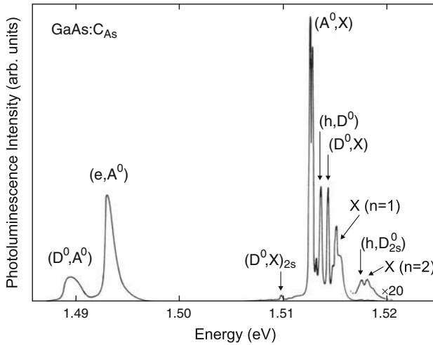
Fig. 10.8 Photoluminescence spectrum ( T = 2 K, D = 10 mW cm -2 ) of GaAs:C As ( N_A = 10^{14} cm -3 ) with donor- and acceptor-related bound-exciton recombination around 1.512 eV, (e, A^0) , (h, D^0) and (D^0, A^0) pair and free-exciton recombination. Adapted from [840]
