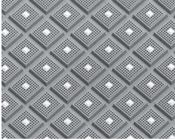
Fig. 22.10 Part of a 256 \times 256 QWIP focal plane array (FPA) with grating coupler (area of one pixel: 37 \mu\text{m}^2 ). From [1543]
