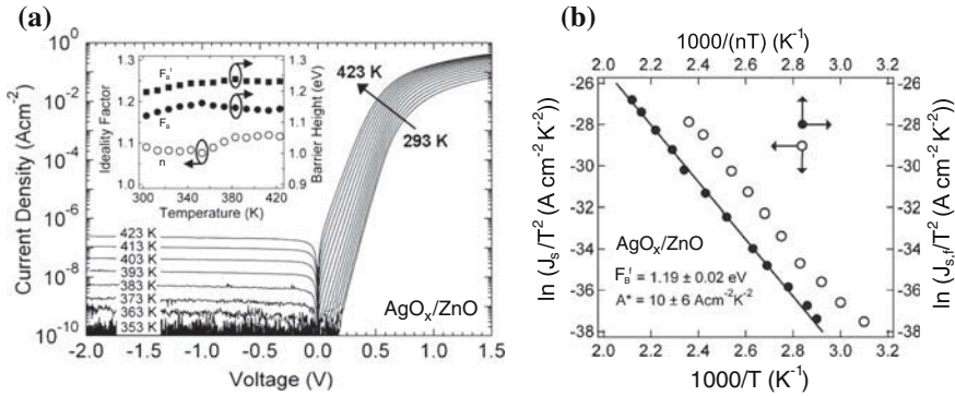
Fig. 21.14 Temperature dependent behavior of an \text{AgO}_x/\text{ZnO} Schottky diode. (a) I - V -characteristics. Inset depicts extracted parameters, ideality factor n , barrier height F_B and flatband barrier height F_B^f (21.54). (b) Richardson plots for the extracted barrier height and the calculated flatband barrier height with linear fit. Adapted from [1440]
