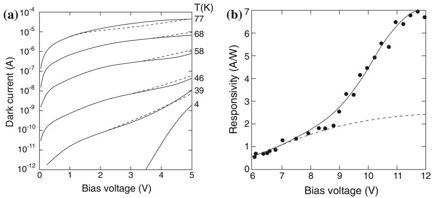
Fig. 22.11 (a) Dark current of a QWIP at 10.7\mu\text{m} , experimental ( solid lines ) and theoretical ( dashed lines ) response. (b) QWIP responsivity as a function of the applied voltage. The solid line ( dashed line ) is the theoretical dependence with (without) the effect of avalanche multiplication. Adapted from [1540]
