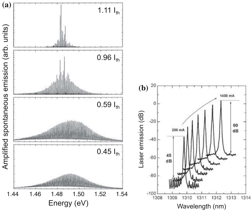
Fig. 23.50 (a) Mode spectra of a Fabry–Perot laser, under, at and above threshold ( I_{\text{thr}} = 13.5 mA). Adapted from [1047]. (b) Mode spectra of a cw DFB InGaAs/InP laser with 2 mm cavity length at various currents of 200, 400, . . . , 1400 mA ( I_{\text{thr}} = 65 mA), SSR > 40 dB at T = 293 K. Adapted from [1697], reproduced with permission from SPIE
