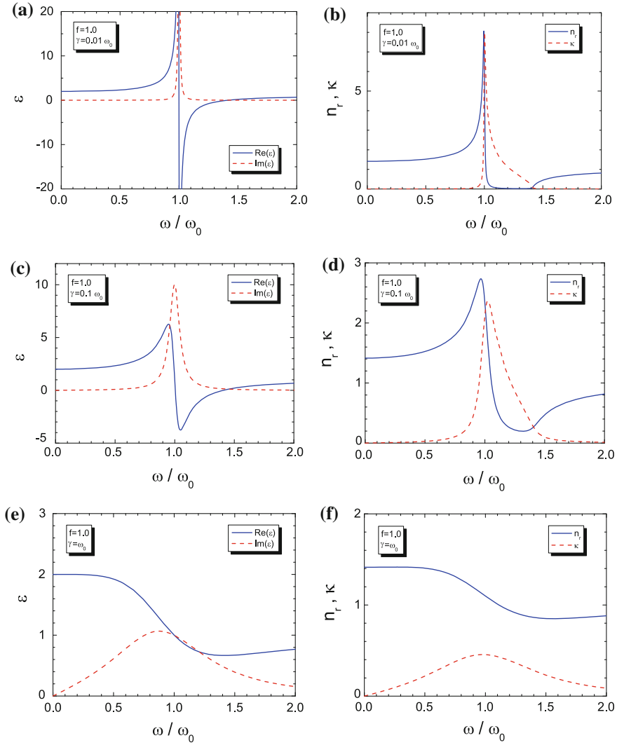
Fig. D.1 Real (solid lines) and imaginary (dashed lines) parts of the dielectric constant ( a, c, e ) and index of refraction ( b, d, f ) (D.11) for oscillator strength f = 1 and various values of damping: ( a, b ) \Gamma = 10^{-2}\omega_0 , ( c, d ) \Gamma = 10^{-1}\omega_0 , and ( e, f ) \Gamma = \omega_0
