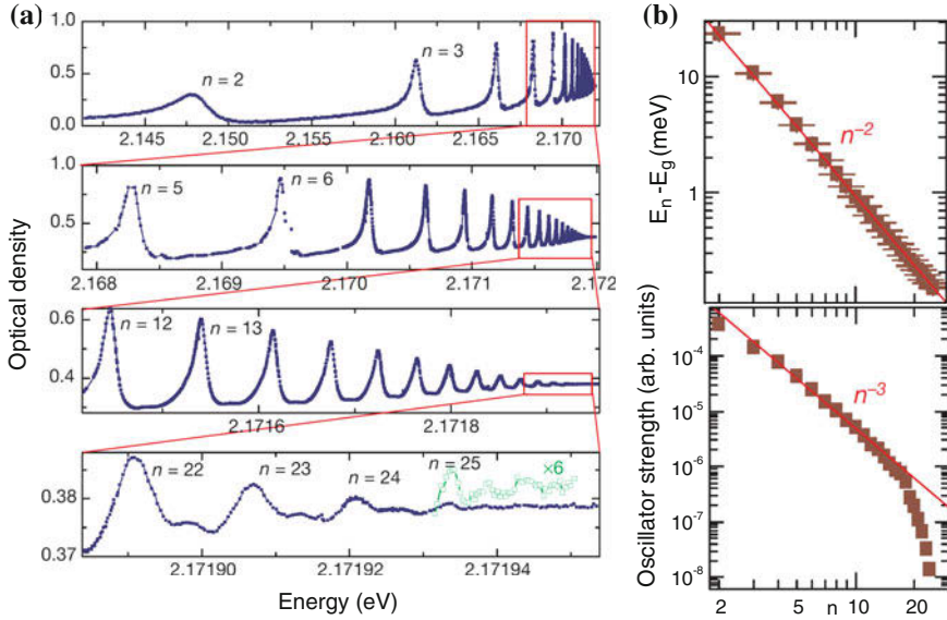
Fig. 9.18 (One photon) Absorption spectrum of Cu 2 O (thickness 34 \mu m) at T = 1.2 K with transitions labelled n = 2 \dots 25 . Adapted from [751]
