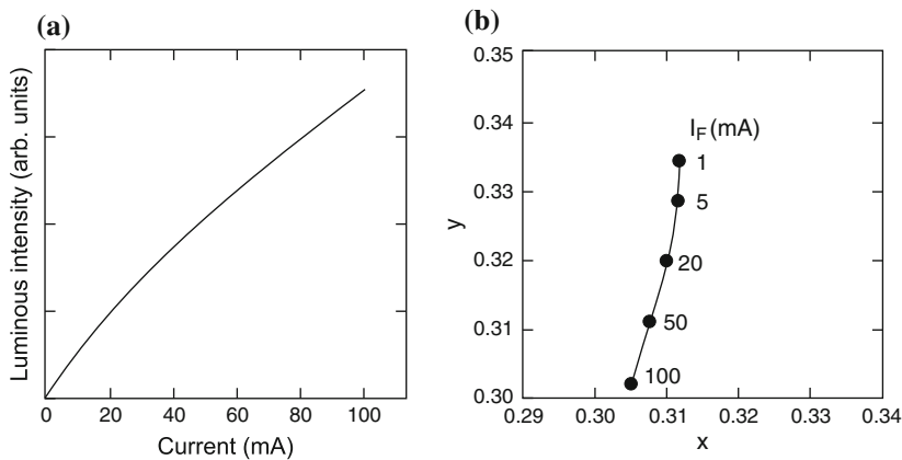
Fig. 23.21 (a) Luminous intensity of white LED (NSCW215) versus dc forward current. (b) CIE chromaticity coordinates for various dc driving conditions as labeled. Data taken from [1657]
