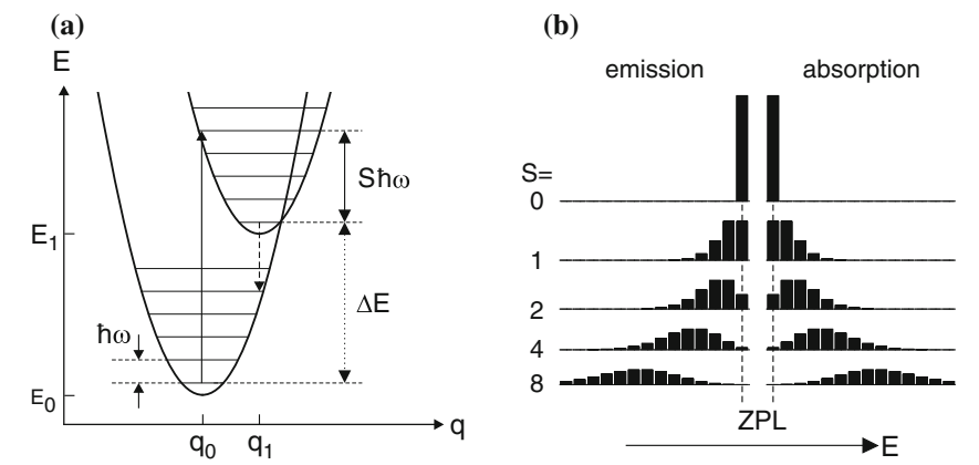
Fig. 10.21 (a) Configuration diagram of two states that differ in their configuration coordinate by \delta q = q_1 - q_0 . Both are coupled to phonons of energy \hbar\omega . The absorption maximum ( solid vertical line ) and emission maximum ( dashed vertical line ) are shifted with respect to the zero-phonon line ( dotted vertical line ) with energy E_1 - E_0 . The Huang–Rhys parameter is S \sim 4 . (b) Intensity of zero-phonon line (‘ZPL’) and phonon replica (10.35) for emission and absorption processes with different values of the Huang–Rhys parameter S as labeled
