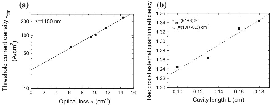
Fig. 23.45 (a) Threshold current density for (three-fold InGaAs/GaAs QD stack) laser ( \lambda = 1150 \text{ nm} ) at 10^\circ\text{C} with different cavity length versus the optical loss ( \propto 1/L ). The extrapolated transparency current density is 21.5 \pm 0.9 \text{ A}/\text{cm}^2 . (b) Inverse external quantum efficiency versus cavity length. The internal quantum efficiency determined from the plot is 91 % and the internal loss is 1.4 \text{ cm}^{-1}
