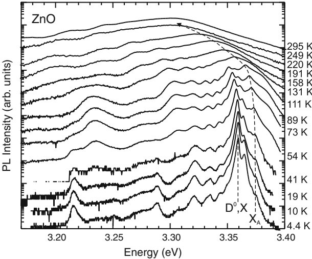
Fig. 10.5 Temperature-dependent luminescence spectra of a ZnO thin film (on sapphire). At low temperatures, the spectra are dominated by donor-bound exciton transitions ( \text{Al}^0 , \text{X} ). The vertical dashed line indicates the low-temperature position of the donor-bound exciton transition ( \text{D}^0 , \text{X} ). The curved dashed line visualizes the energy position of the free-exciton transition ( \text{X}_\text{A} ) that becomes dominant at room temperature
