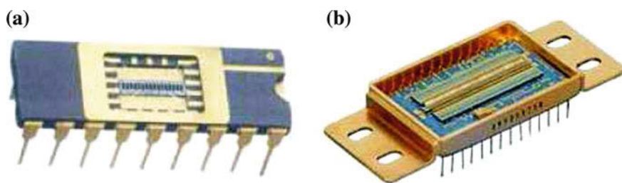
Fig. 22.48 (a) Array of 16 silicon APDs. From [1575]. (b) 1024-pixel InGaAs photodiode array. From [1576]
