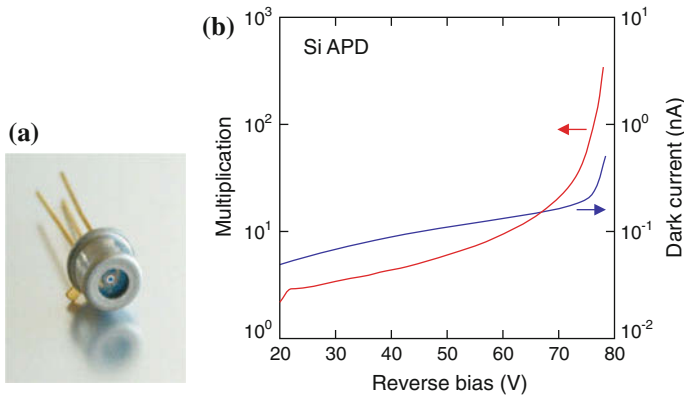
Fig. 22.31 (a) TO casing of Si APD. (b) Dark current ( blue ) (active area 0.2 \text{ mm}^2 ) and multiplication factor ( red ) as a function of reverse bias (at 23^\circ\text{C} ). Adapted from [1556]
