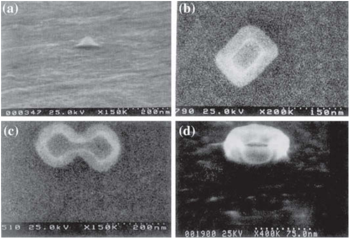
Fig. 14.22 Quantum dots of various shapes created by lithography and etching techniques. From [1163]
