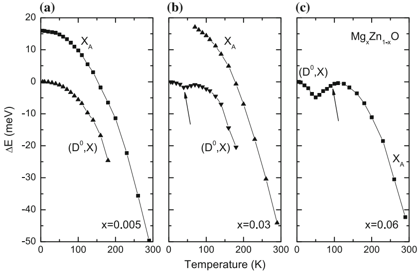
Fig. 10.17 Temperature dependence of the shift of energy position of (D^0, X) and X_A photoluminescence peak in Mg_x Zn_{1-x}O alloys with three different Mg-contents, (a) x = 0.005 , (b) x = 0.03 , (c) x = 0.06 . The energy positions are given relative to the low temperature position of the respective (D^0, X) peaks. Adapted from [860]
