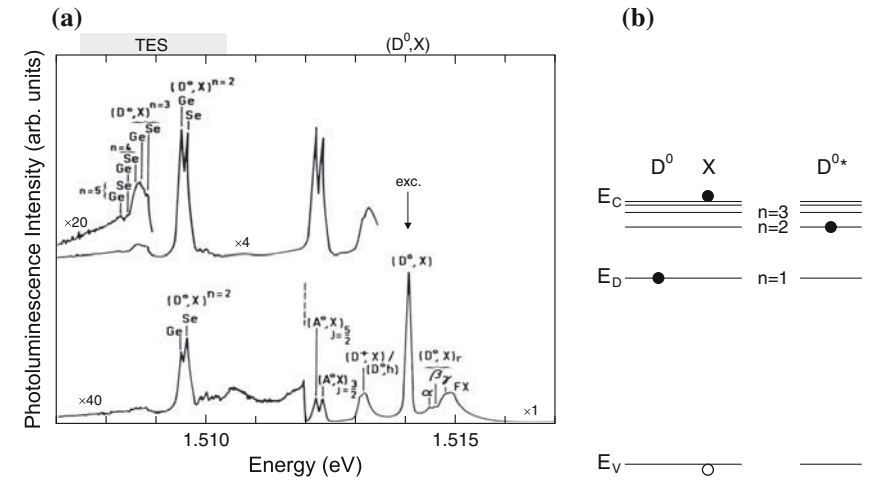
Fig. 10.10 (a) Photoluminescence spectrum ( T = 1.5 K, D = 50 mW cm ^{-2} ) of high-purity GaAs with two donors (Ge and Se/Sn). The lower spectrum has been excited 6 meV above the band gap, the upper spectrum has been resonantly excited with the laser set to the (D^0, X) transition and exhibits n = 2, 3, 4 , and 5 TES transitions. \alpha , \beta , \gamma denote excited (hole rotational) states of the (D^0, X) complex. Adapted from [852]. (b) Schematic representation of the n = 2 TES process, left initial, right final state
