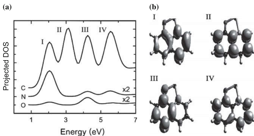
Fig. 17.11 (a) Projected density of states (for C, N, and O) of excited states in an \text{Alq}_3 molecule. The origin of the energy axis is the HOMO level. (b) Orbitals for the four states labeled I–IV in (a). Reprinted with permission from [1253], © 1998 AIP
