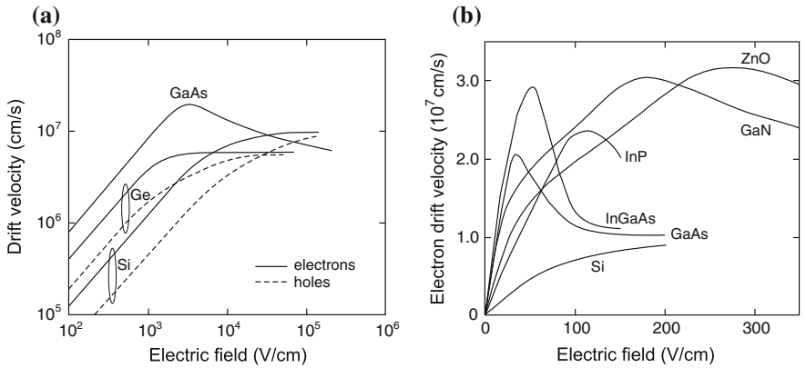
Fig. 8.10 Drift velocity at room temperature as a function of applied electric field for (a) high-purity Si, Ge, and GaAs on a double-logarithmic plot and (b) on linear plots for Si [668], Ge [669], GaAs [598], InP [670], InGaAs [671], GaN and ZnO [672]
