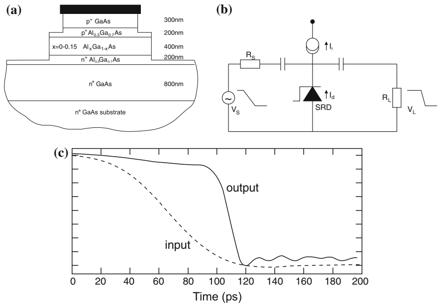
Fig. 21.69 (a) Schematic layer sequence for fast GaAs/AlGaAs step-recovery diode. (b) Circuit with input and output pulse. (c) Input (dashed line) and output (solid line) waveforms. Vertical division is 2 V. Adapted from [1511]
