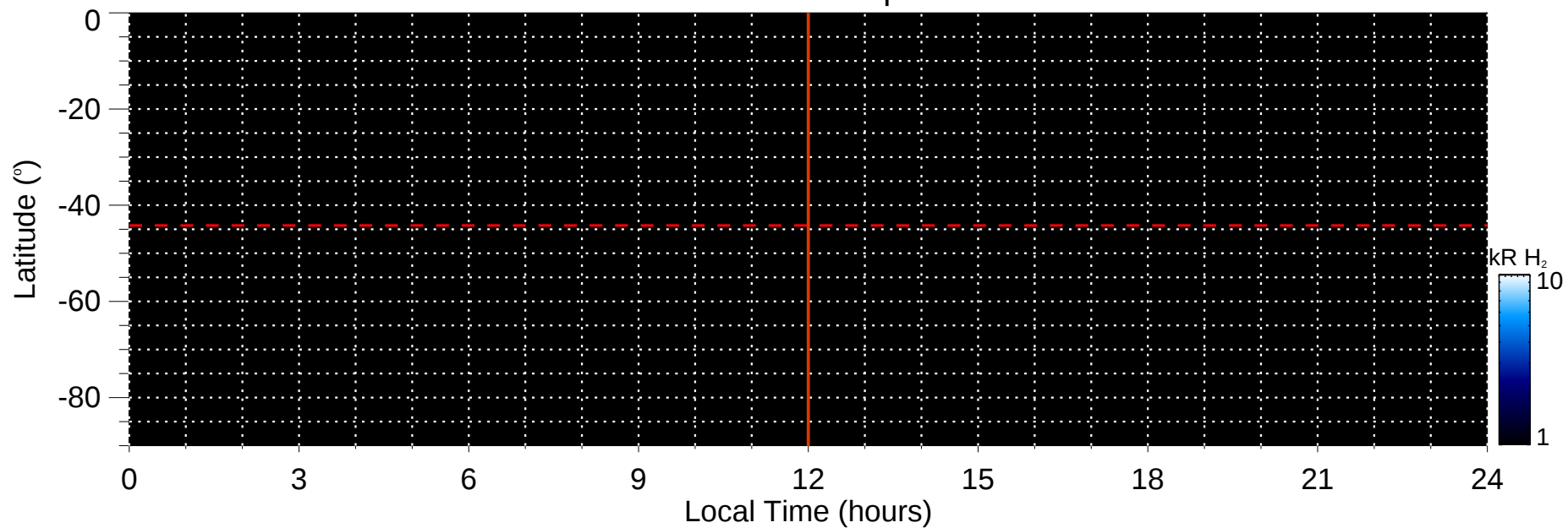
Southern hemisphere
