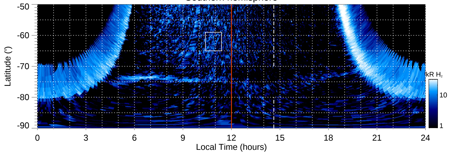
Southern hemisphere
