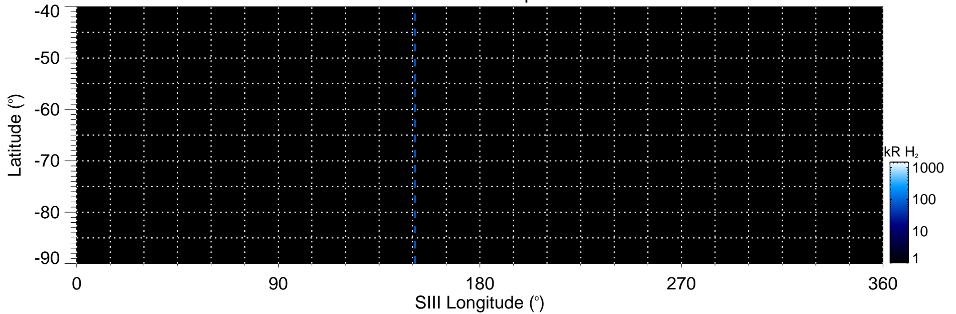
Southern hemisphere
